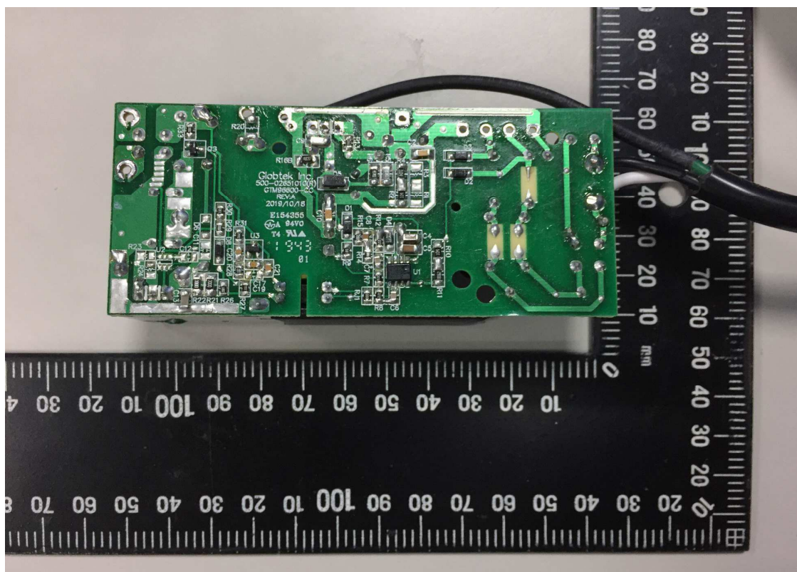
Photo 6 - Bottom view of power board
