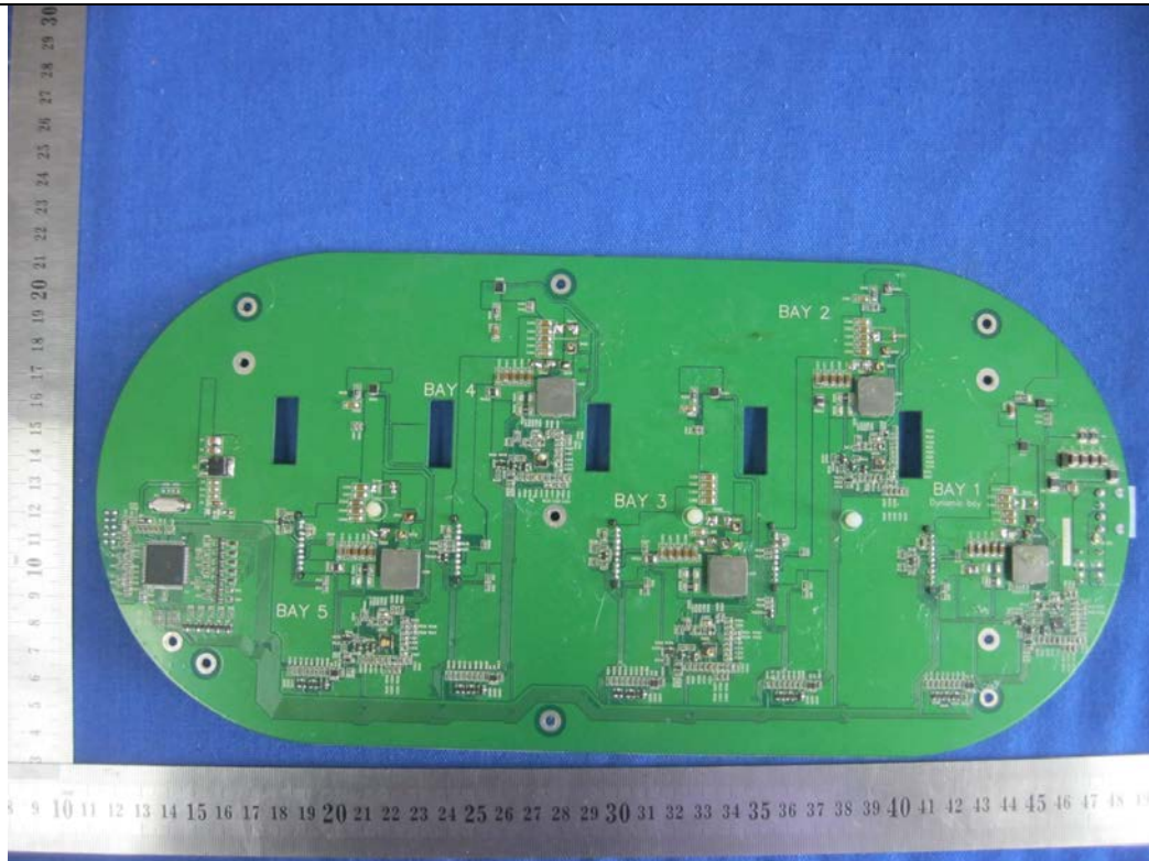
Photo 5: PCB
