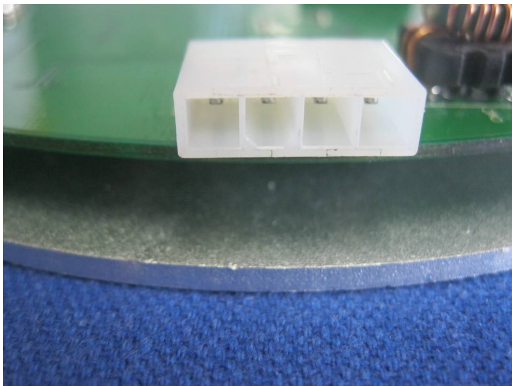
Photo 6: DC-IN connector
