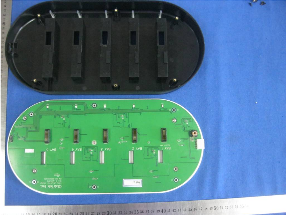
Photo 4: Inner view
