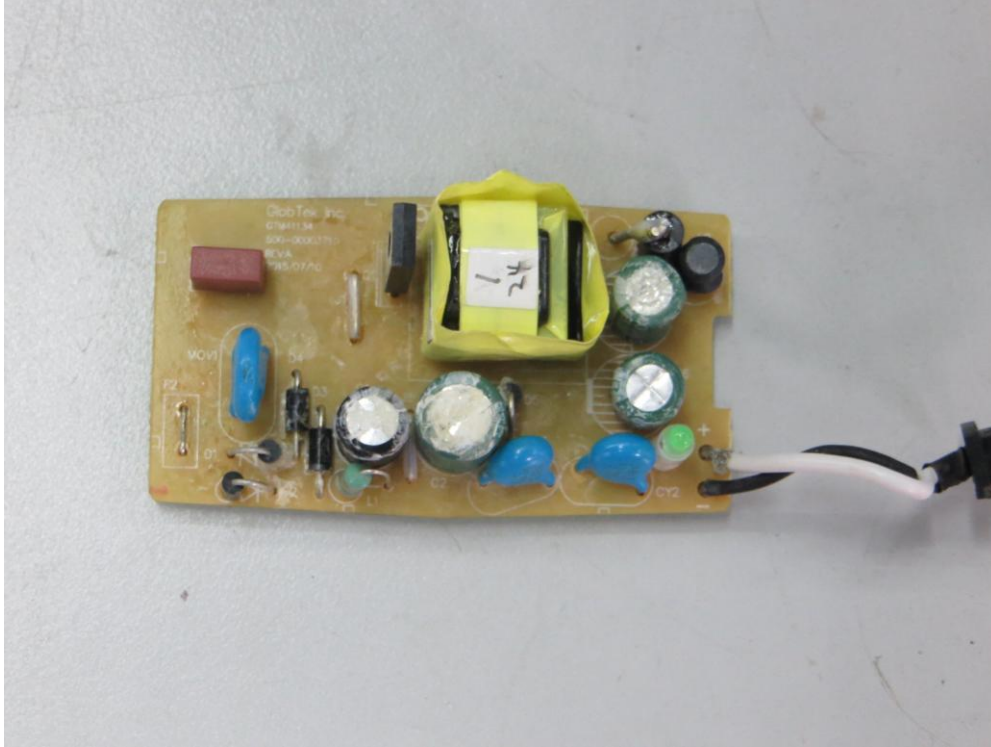
PHOTO 18: COMPONENT SIDE VIEW OF PCB OF MODEL GT*96060*****
