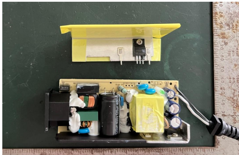
Internal view for GTM96600 series (Class II)
