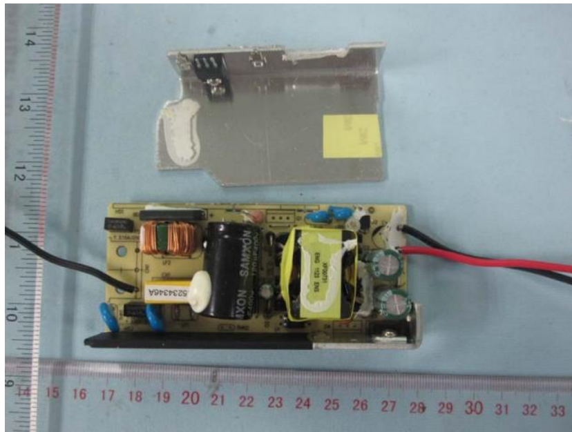
Component side
