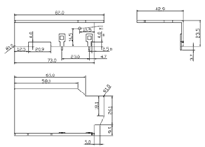
HS1 drawing for GTM96600 series
