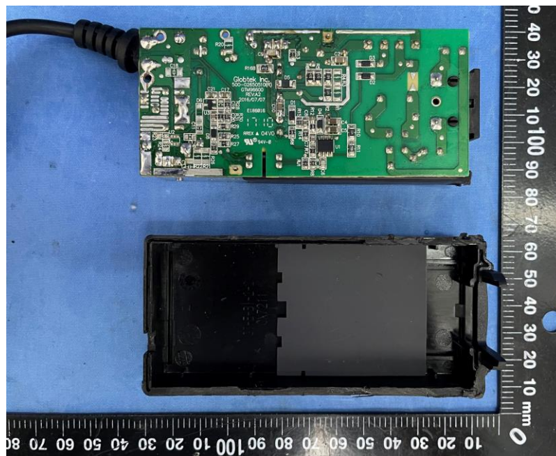
Internal view for GTM96600 series (Class II)
