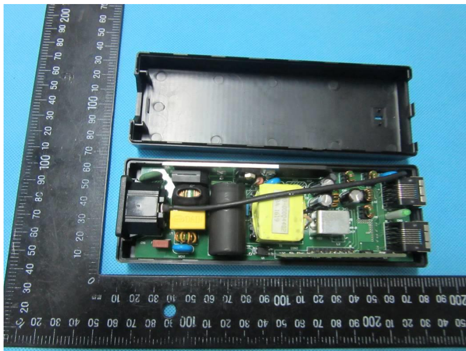
For GT*96600-*56*** (Internal view)
