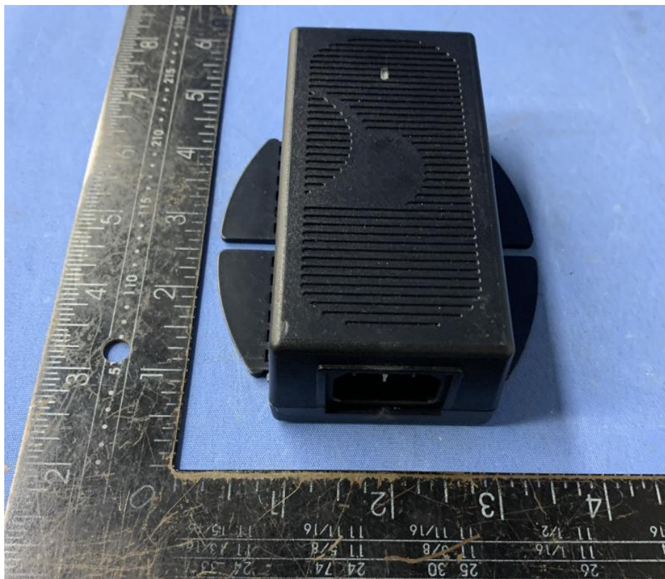
External view for model with POE
