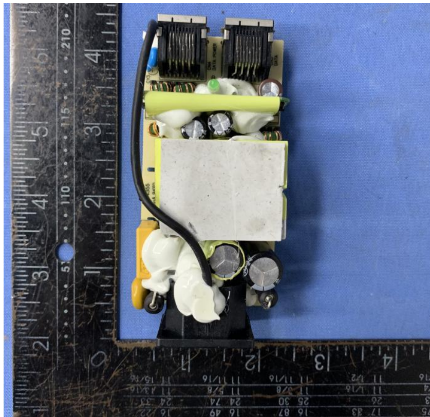
PCB view for model with POE
