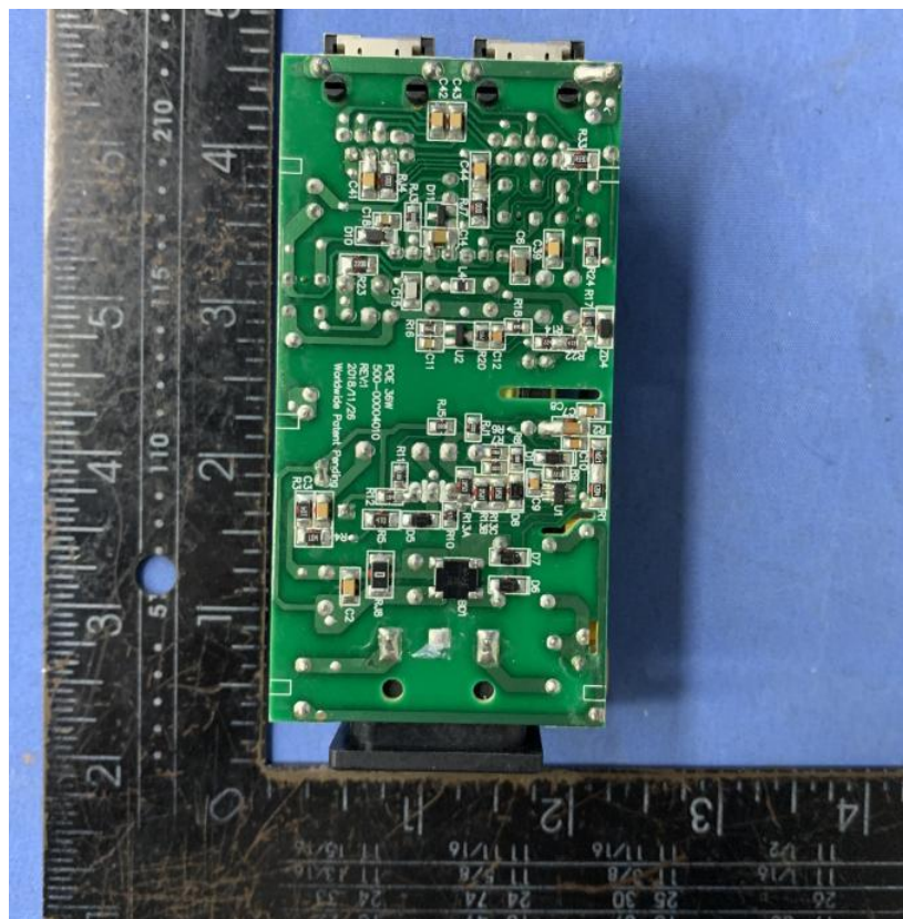
PCB view for model with POE
