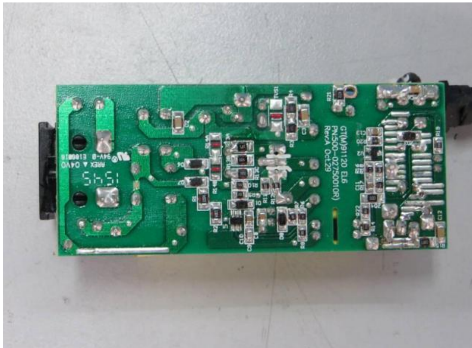
PCB view (Class I)
