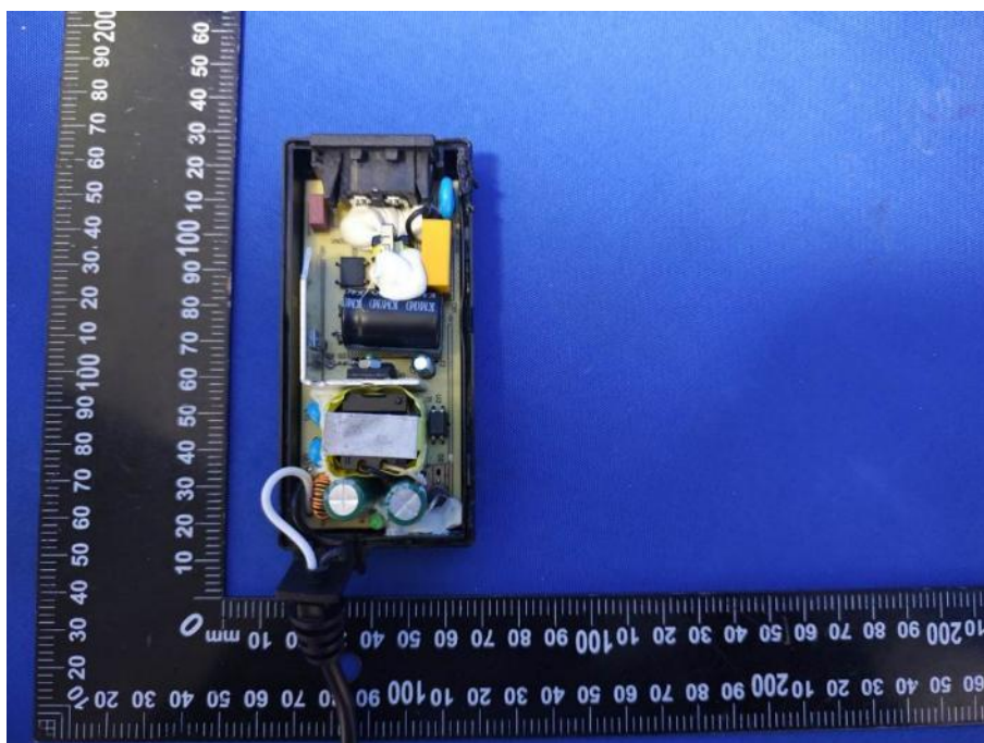
Internal view (without HS2)
