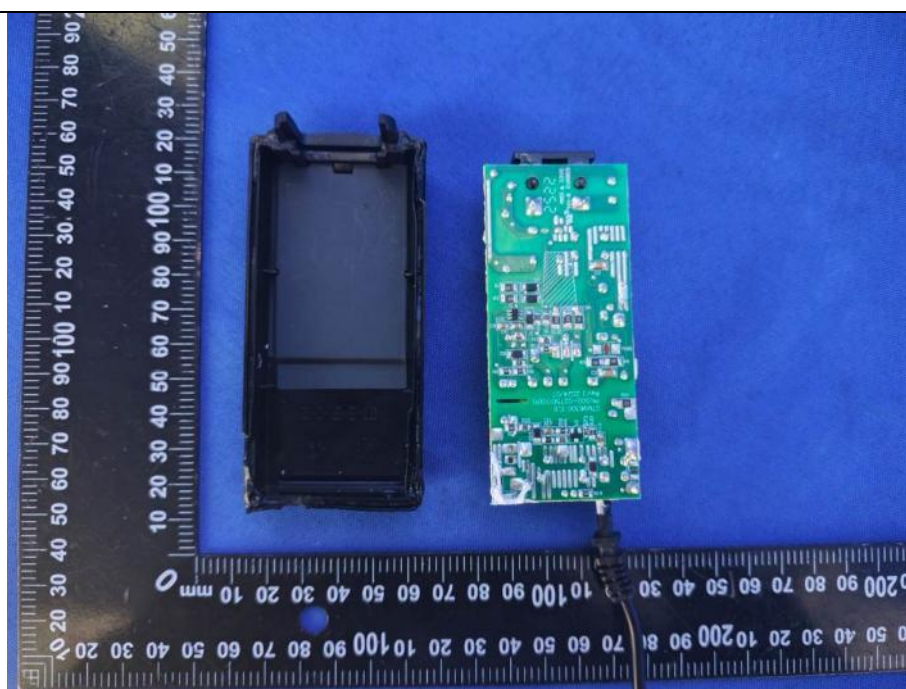
Internal view (plastic enclosure for hybrid desktop)
