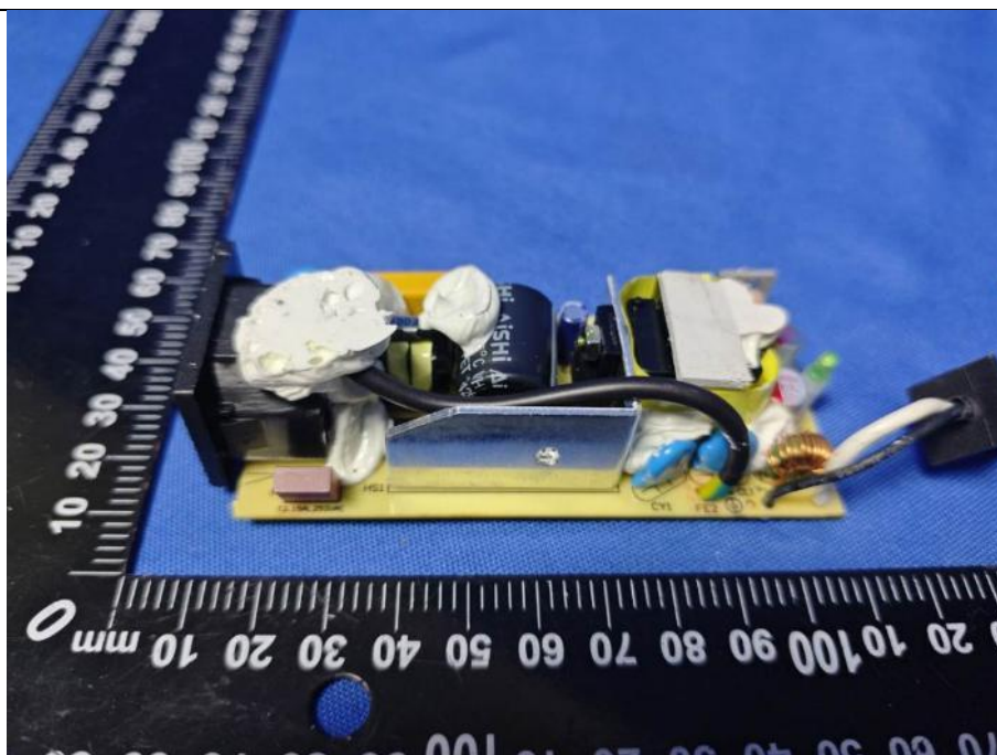
Class I inlet is direct connected to the CY1/CY2 trace
