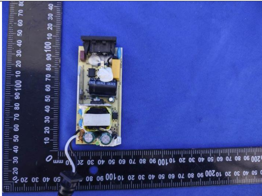
Class II structure
