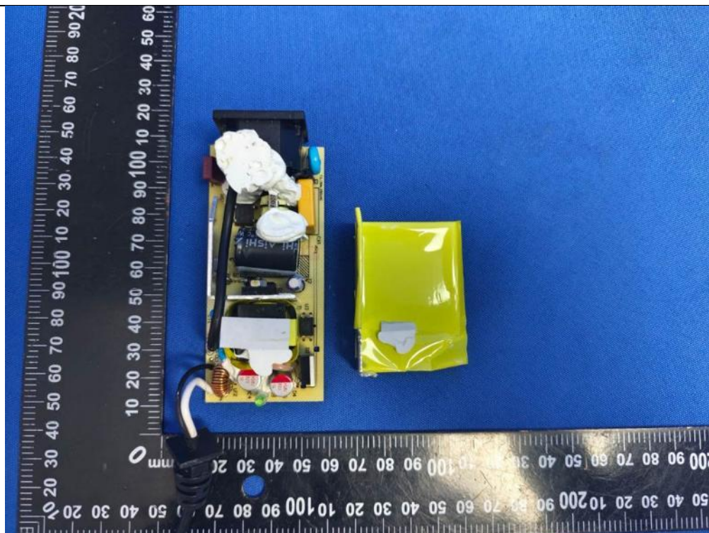
Internal view (with HS2)
