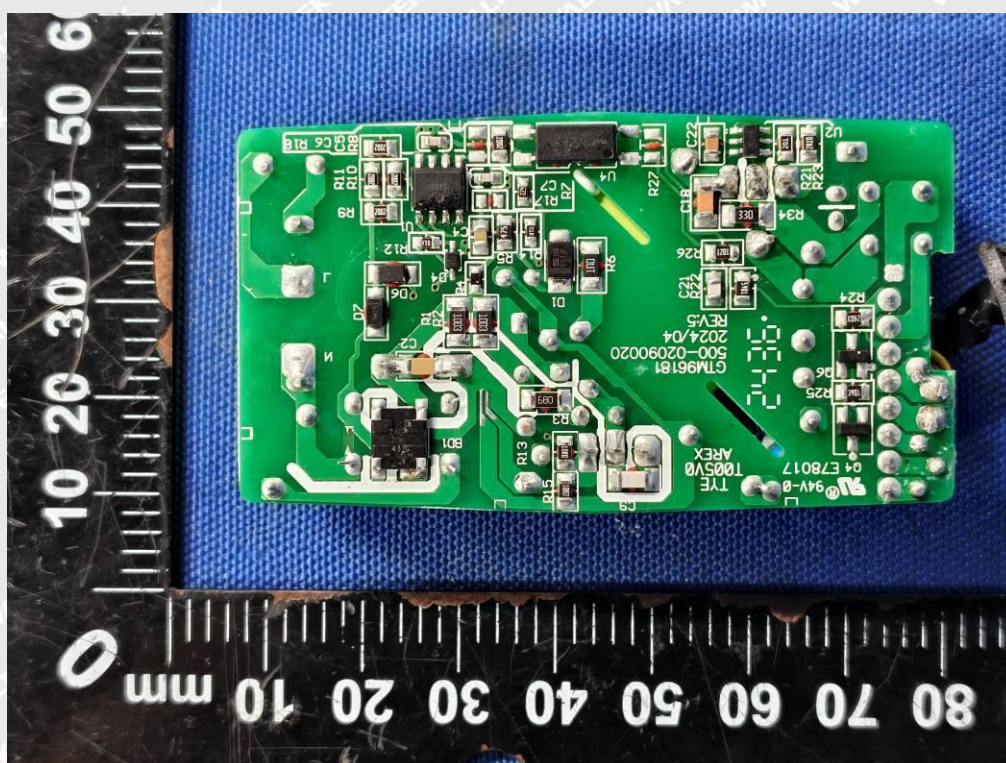
Photo 38 (GTM96181-*PD*** Series - Direct plug-in type with interchangeable plug)
