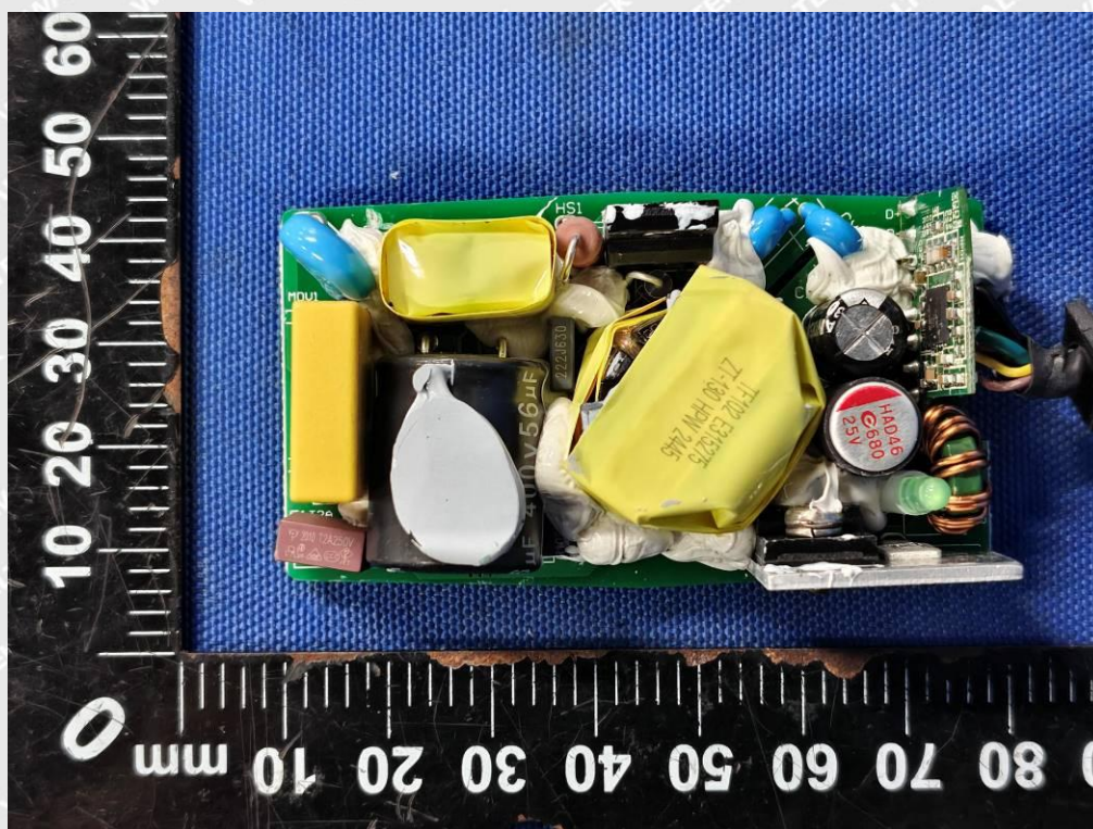
Photo 37 (GTM96181-*PD*** Series - Direct plug-in type with interchangeable plug)
