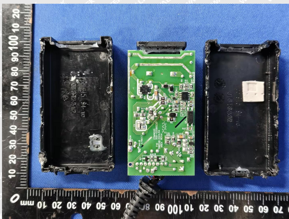
Photo 44 (GTM96181-*PD*** Series - Desk top type with C6 or C14 appliance inlet)
