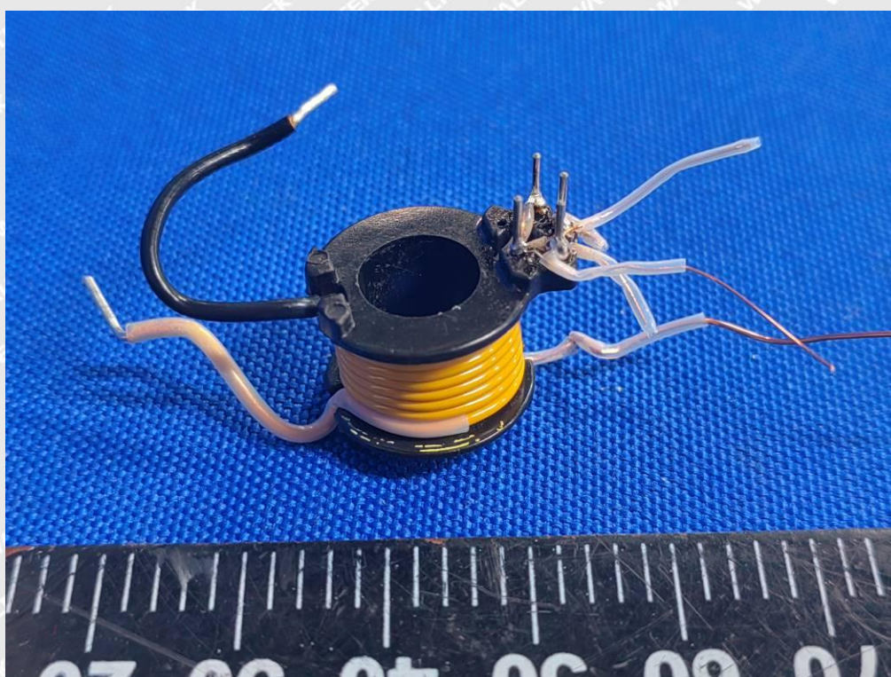
Photo 30 (GTM96183-*PD*-USB1C* Series Transformer – TF123)
