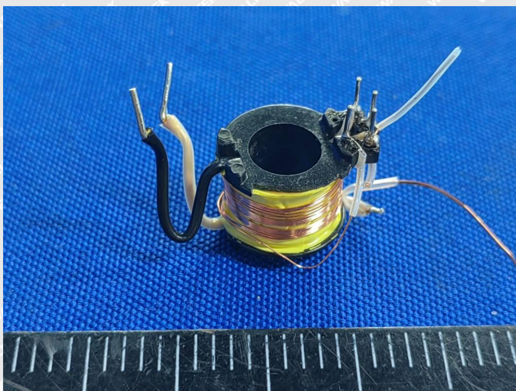
Photo 54 (GTM96181-*PD*** Series Transformer – TF102)
