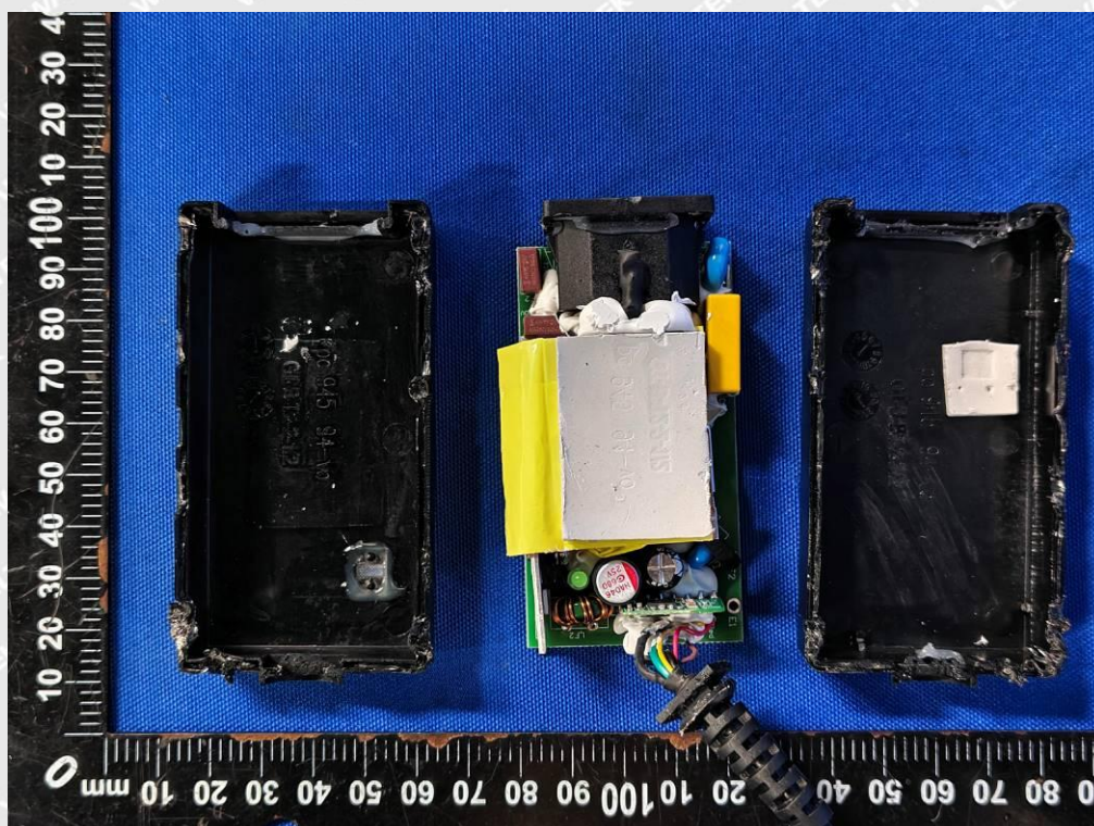
Photo 43 (GTM96181-*PD*** Series - Desk top type with C6 or C14 appliance inlet)
