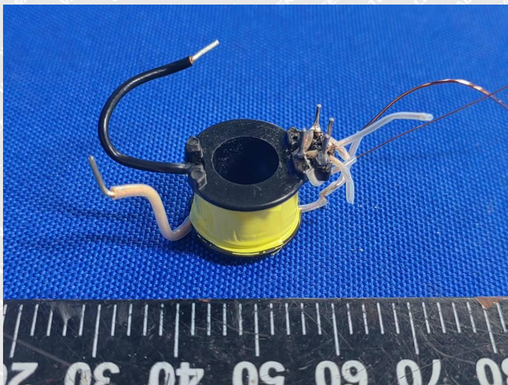
Photo 29 (GTM96183-*PD*-USB1C* Series Transformer – TF123)
