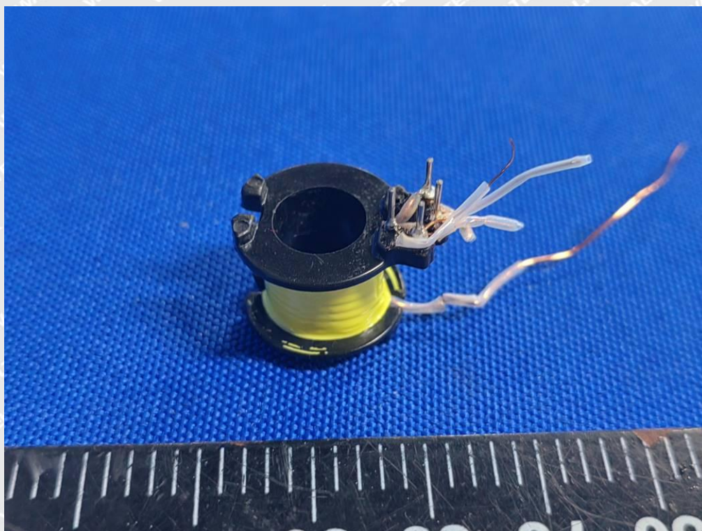
Photo 31 (GTM96183-*PD*-USB1C* Series Transformer – TF123)
