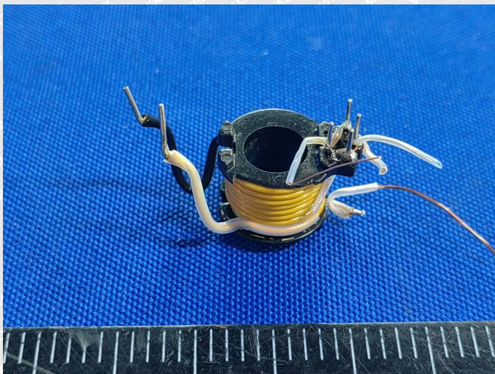
Photo 56 (GTM96181-*PD*** Series Transformer – TF102)
