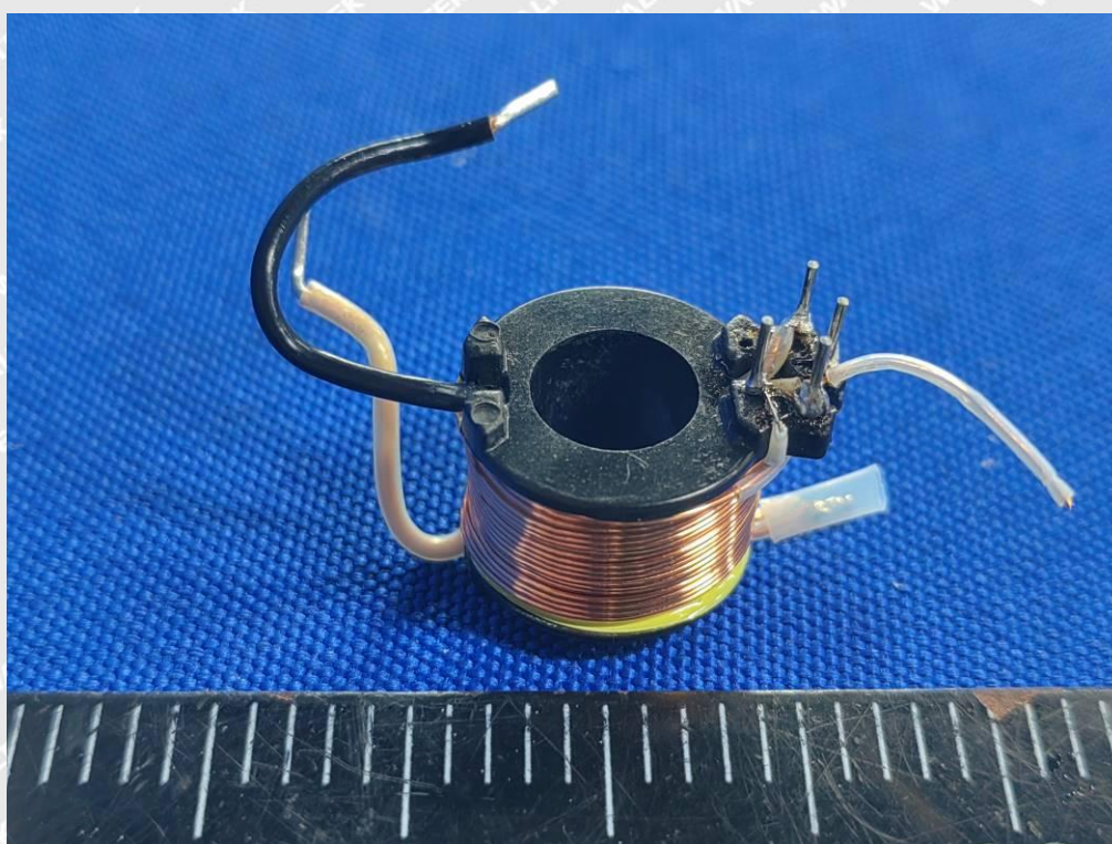
Photo 26 (GTM96183-*PD*-USB1C* Series Transformer – TF123)
