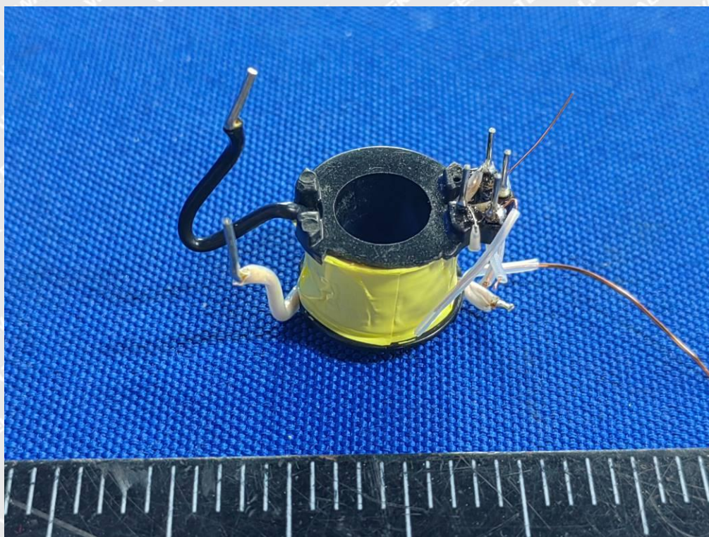
Photo 55 (GTM96181-*PD*** Series Transformer – TF102)
