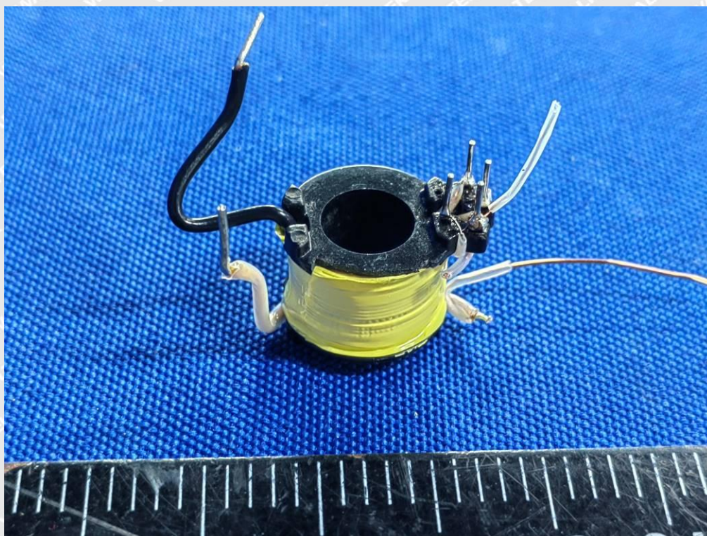
Photo 53 (GTM96181-*PD*** Series Transformer – TF102)
