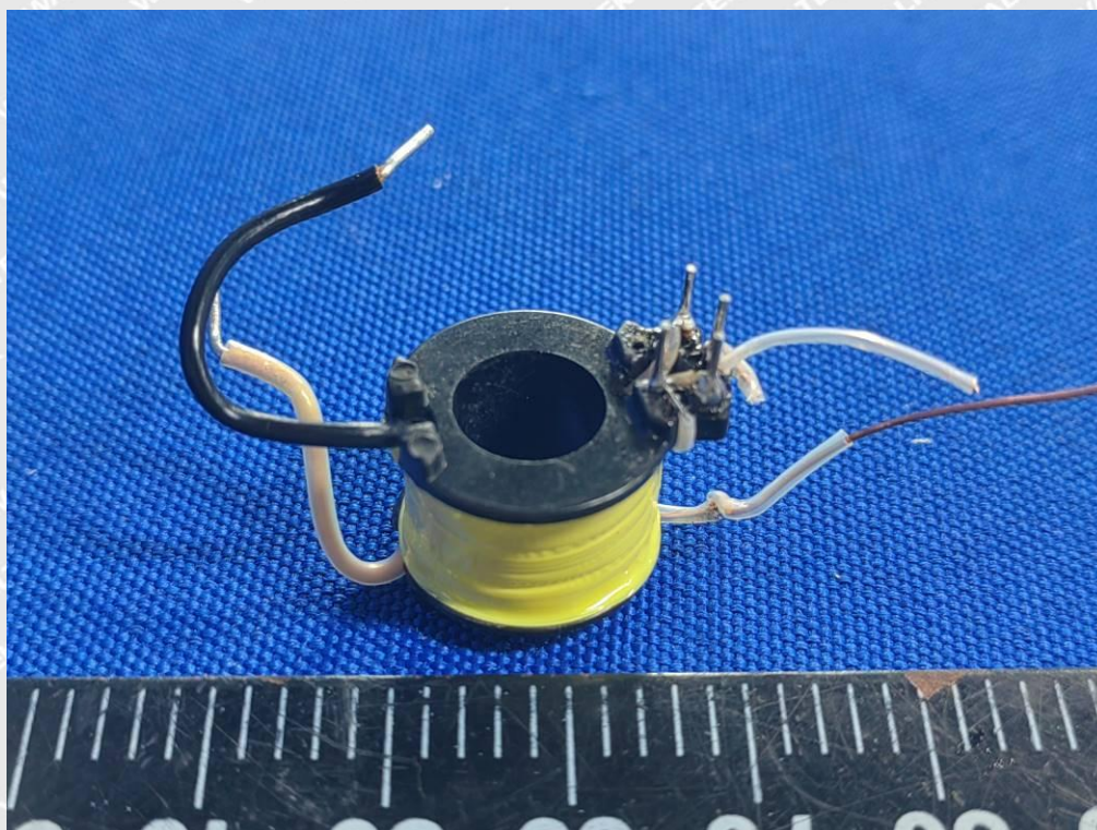
Photo 27 (GTM96183-*PD*-USB1C* Series Transformer – TF123)
