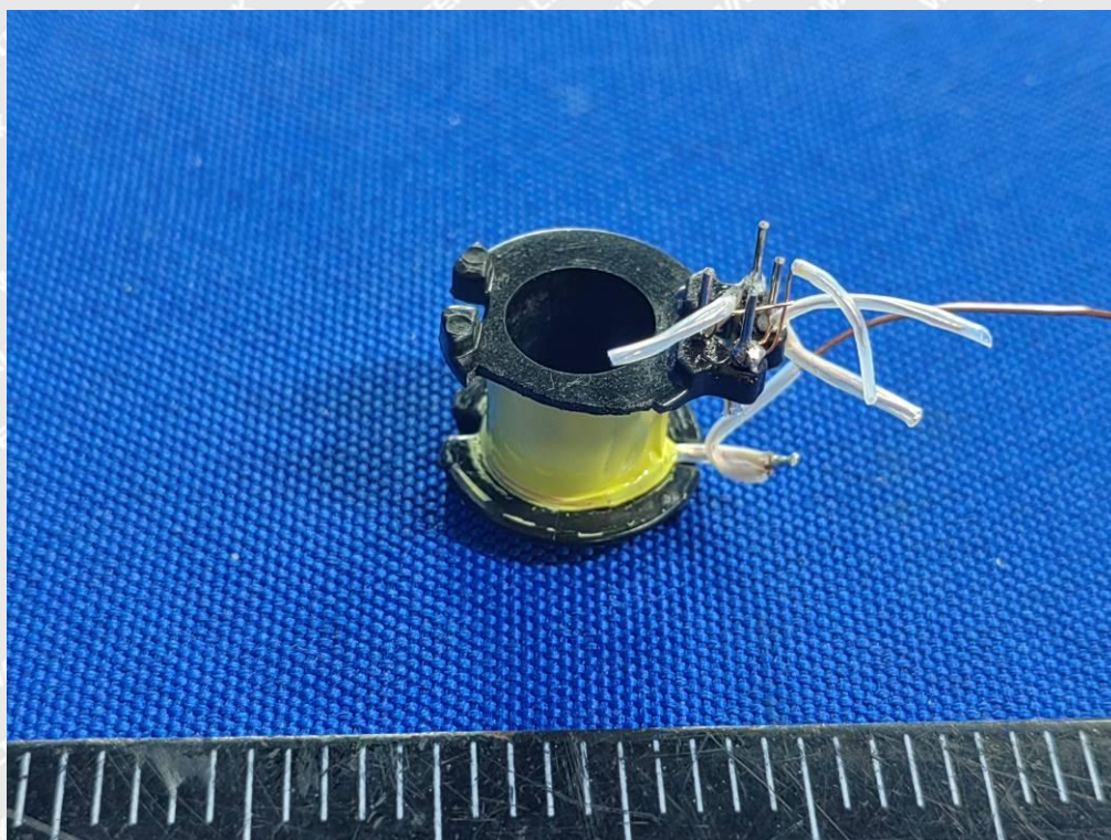
Photo 58 (GTM96181-*PD*** Series Transformer – TF102)
