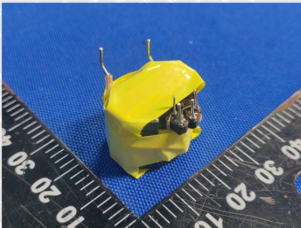
Photo 22 (GTM96183-*PD*-USB1C* Series Transformer – TF123)
