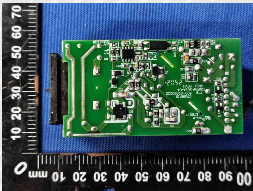
Photo 42 (GTM96181-PD*** Series - Desk top type with C8 AC or C18 AC appliance inlet)
