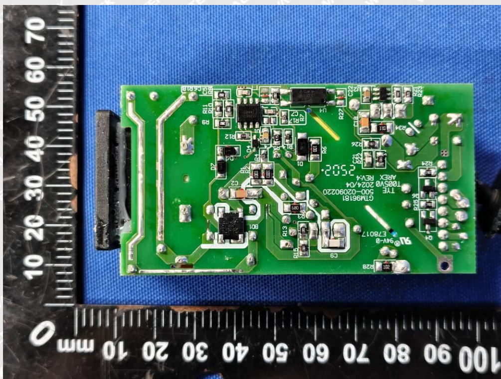
Photo 46 (GTM96181-*PD*** Series - Desk top type with C6 or C14 appliance inlet)
