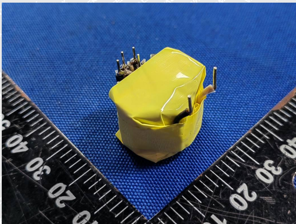
Photo 48 (GTM96181-*PD*** Series Transformer – TF102)
