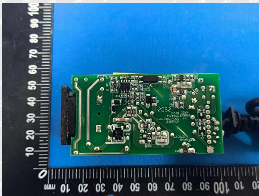
GTM96181-18PD-PPS-T3
