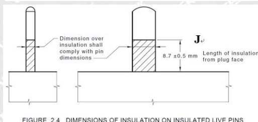
FIGURE 2.4 DIMENSIONS OF INSULATION ON INSULATED LIVE PINS
