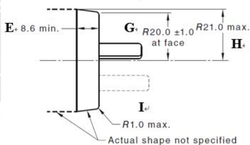
(e2) Shape of plugs having ratings up to 20 A, 250 Vmax. and of the (a1), (a2), (c), (d), (f) or (g) type.
