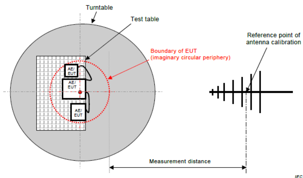
Figure C.1 – Measurement distance
