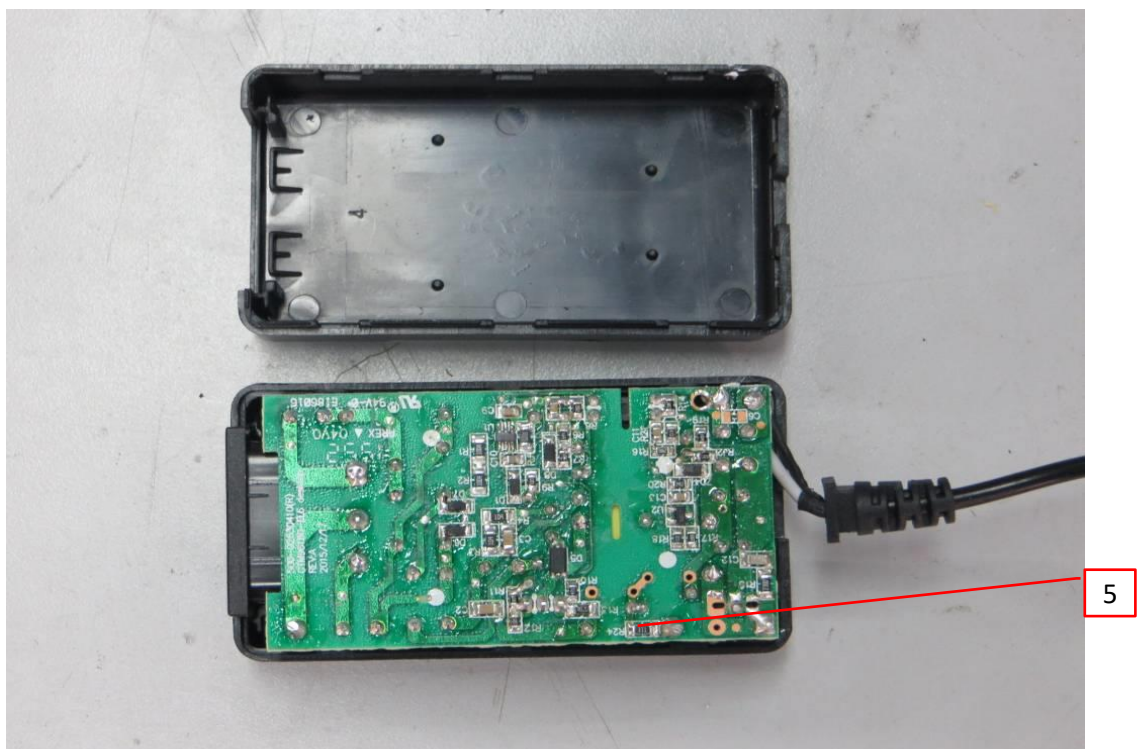
Photo 6 - PCB view for GT*96180 series (Class I)
