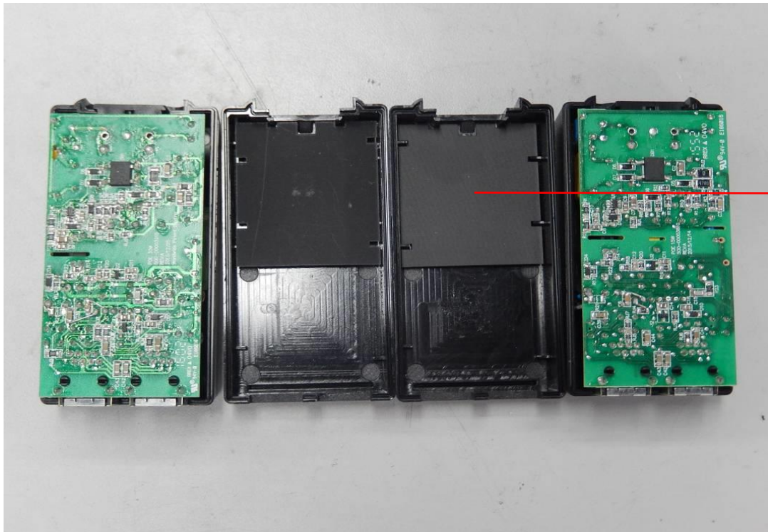
Photo 21 - Internal view for GT*96180 POE series
