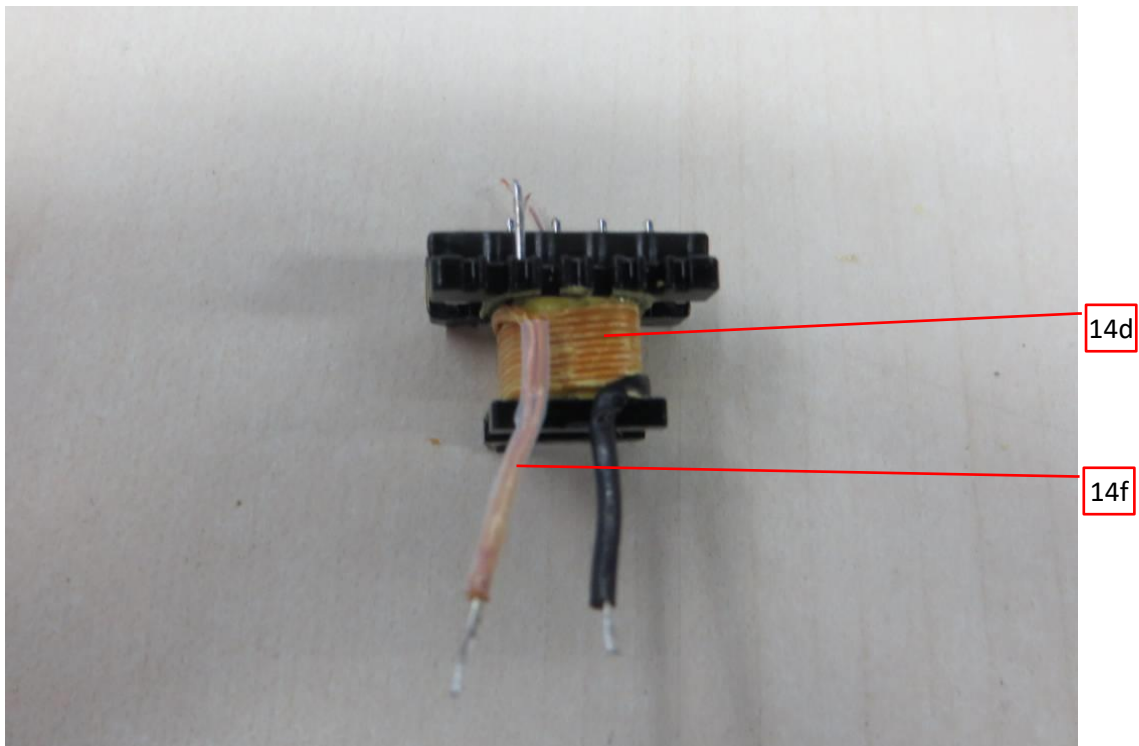
Photo 28 - Transformer
