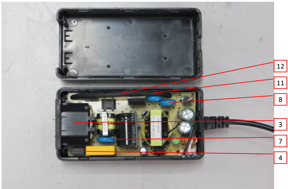
Photo 5 - PCB view for GT*96180 series (Class I)
