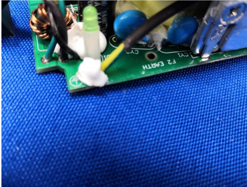
Earthing connection for model GTM961005P-*PD-USBCP-T3A*
