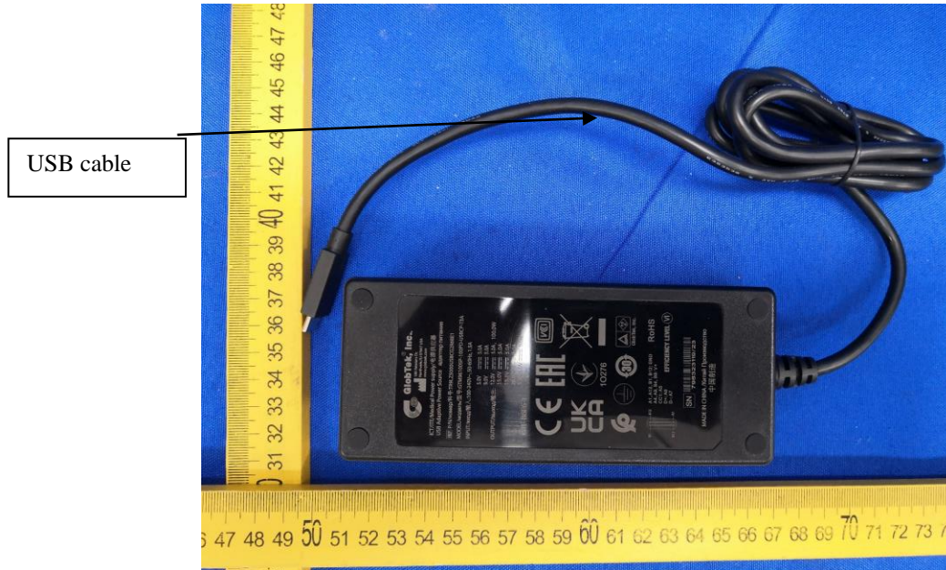
Over view for GTM961005P- *PD-USBCP**
