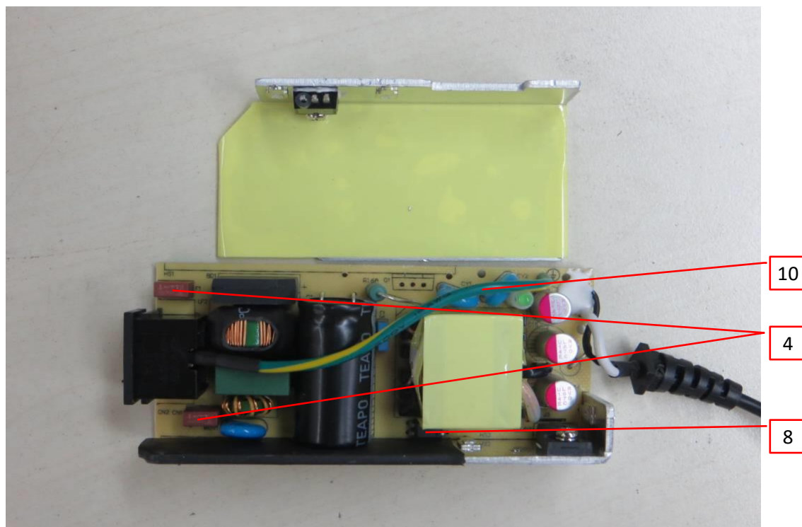
Photo 12 - PCB view
