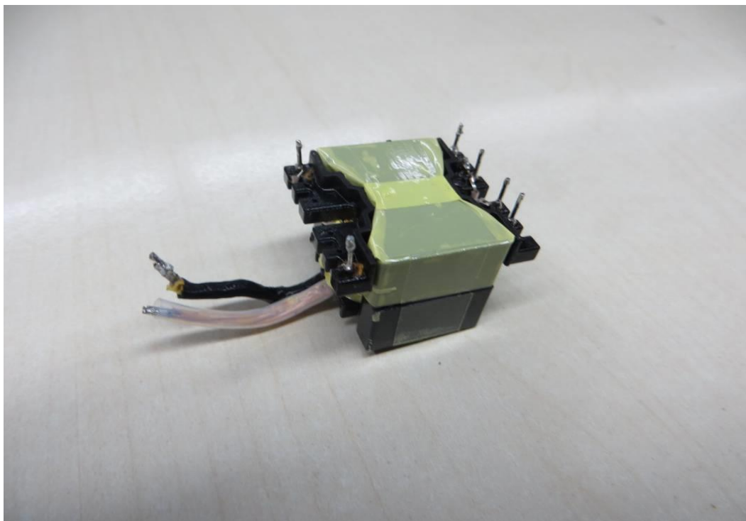
Photo 37 - Transformer for GT*96600-**** series
