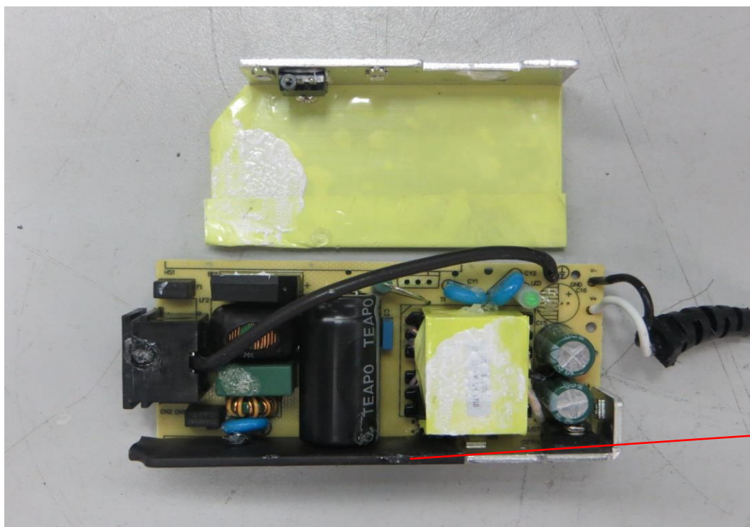
Photo 13 - PCB view
