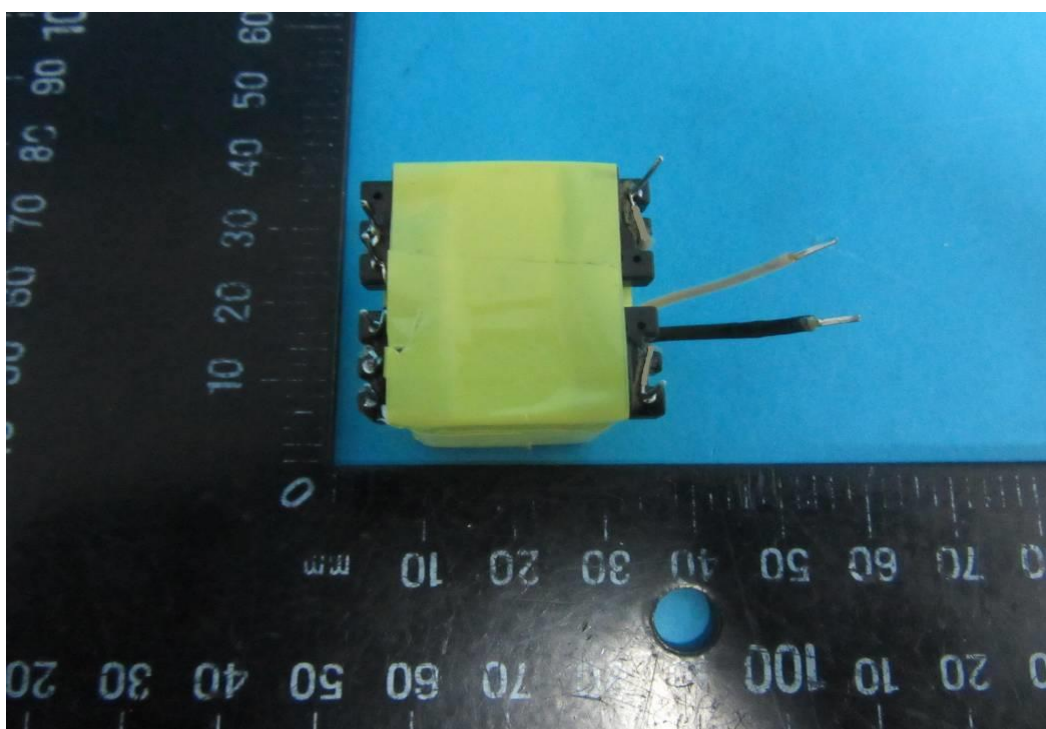
Photo 46 - Transformer for GT*96600-*56*** series
