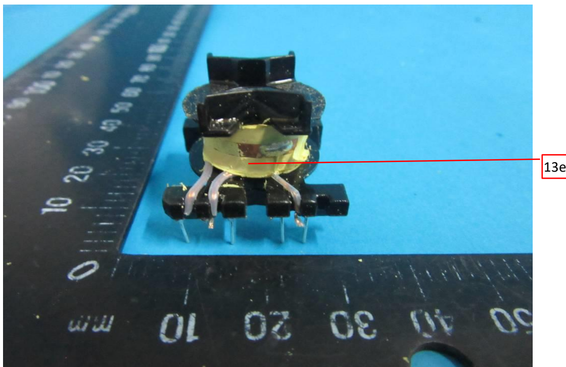
Photo 51 - Transformer for GT*96600-*56*** series
