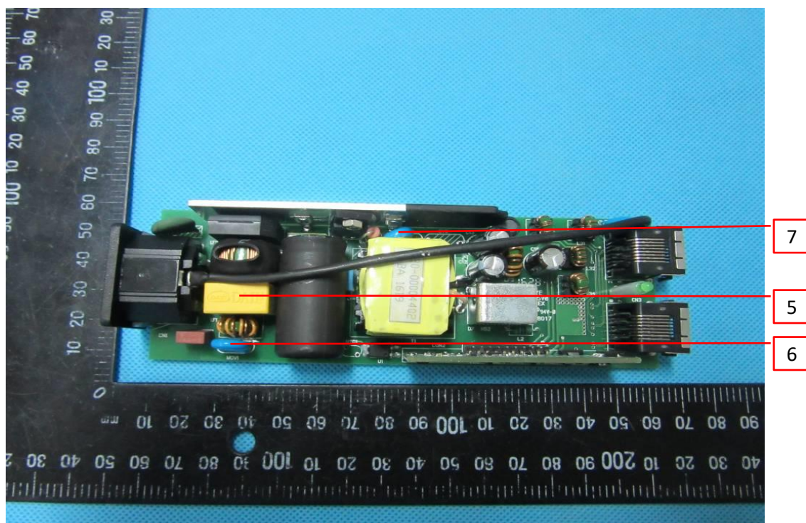
Photo 25 - PCB view
