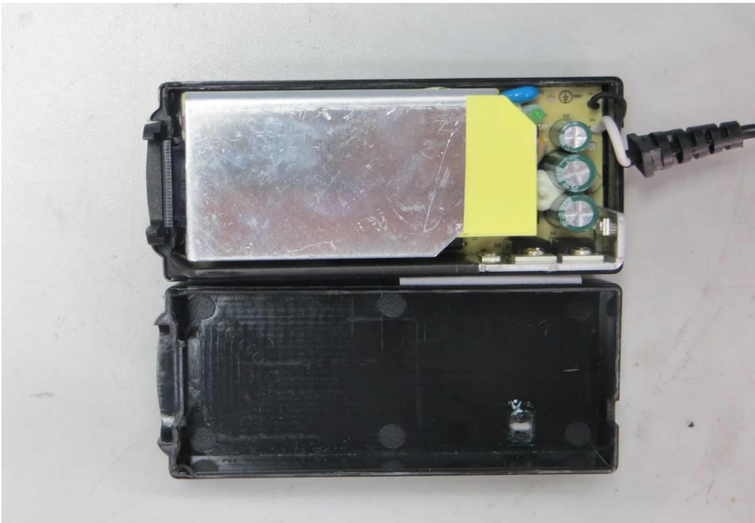
Photo 6 - Internal view
