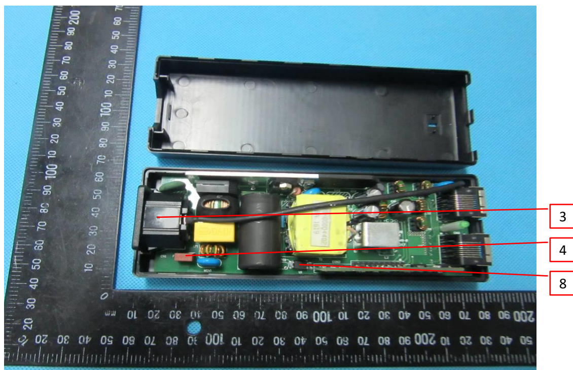
Photo 24 - Internal view
