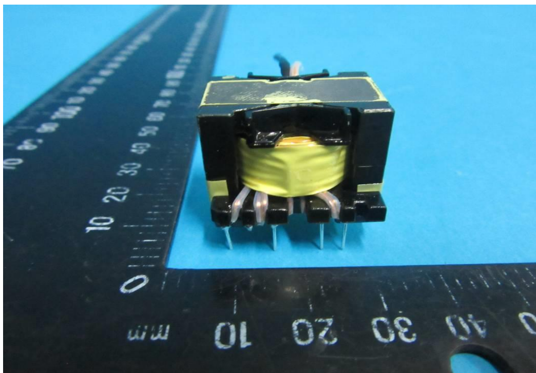
Photo 47 - Transformer for GT*96600-*56*** series
