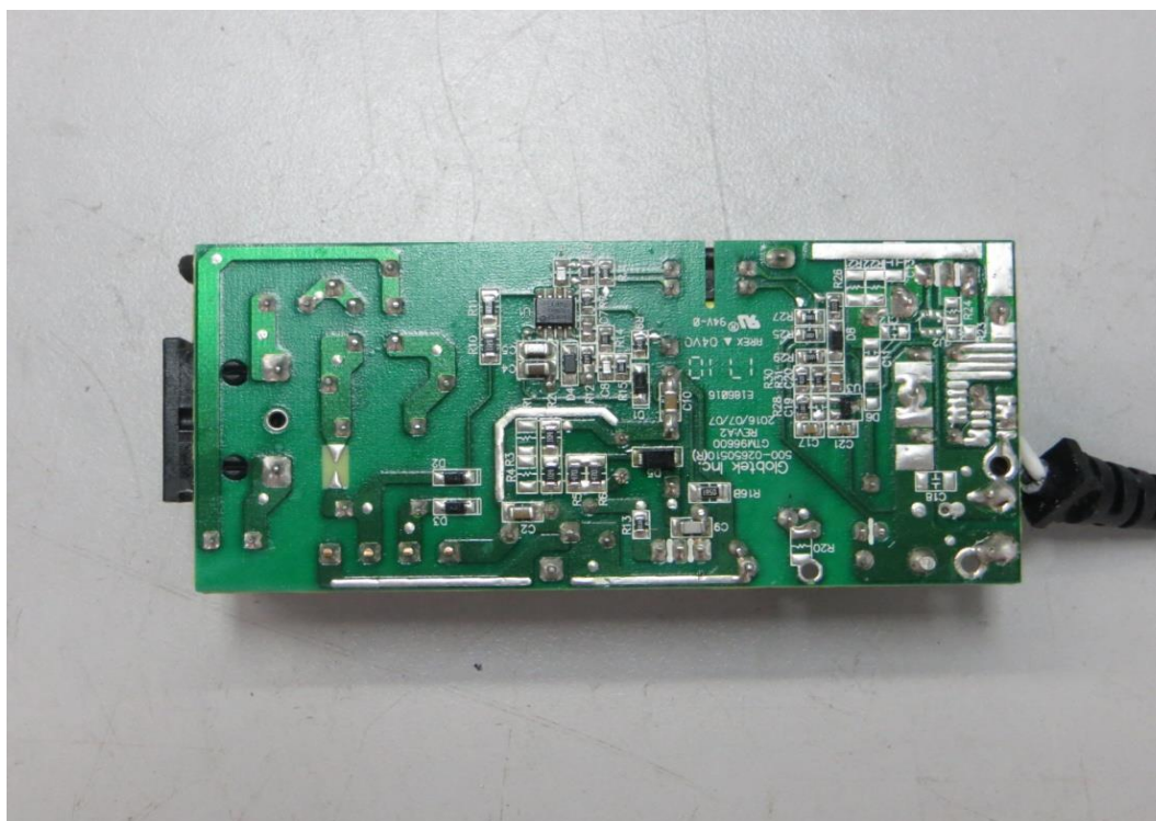
Photo 14 - PCB view
