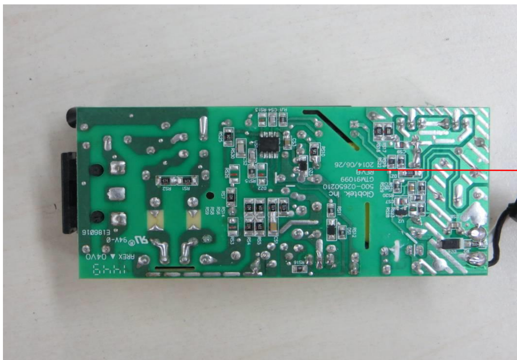
Photo 15 - PCB view
