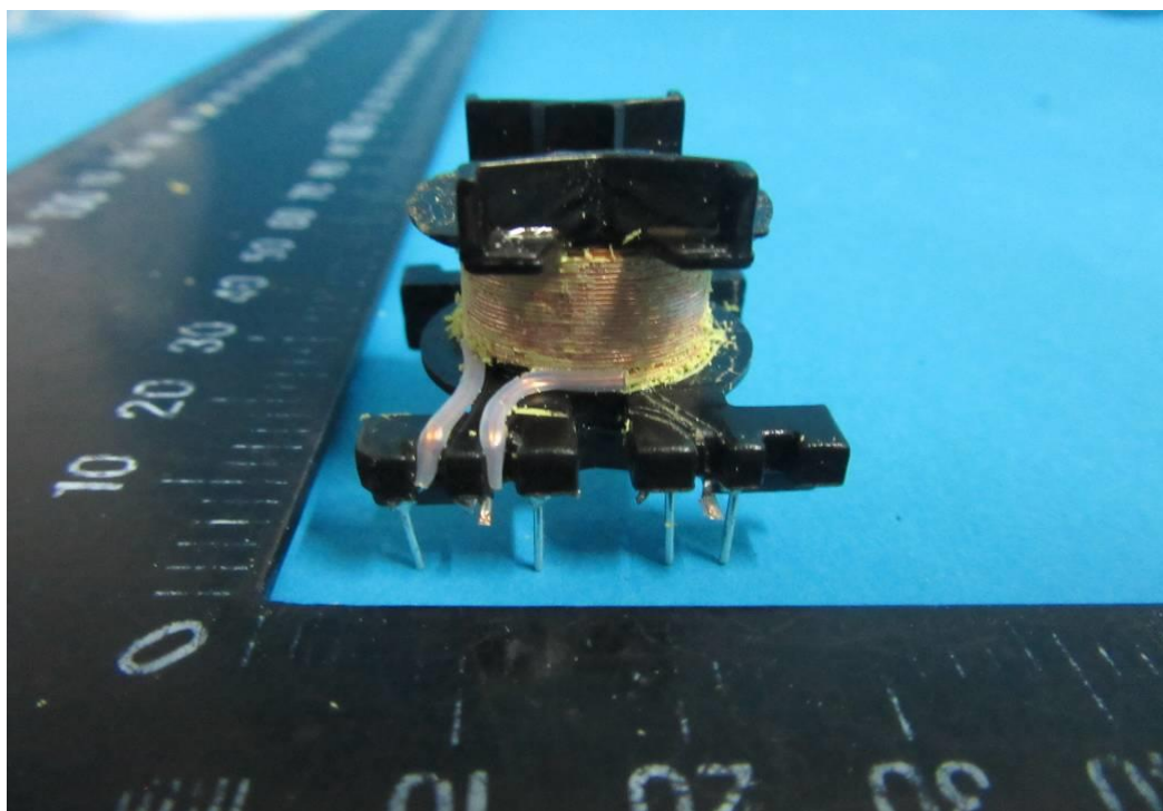
Photo 52 - Transformer for GT*96600-*56*** series
