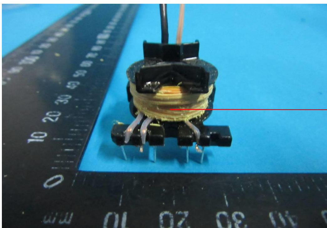
Photo 50 - Transformer for GT*96600-*56*** series
