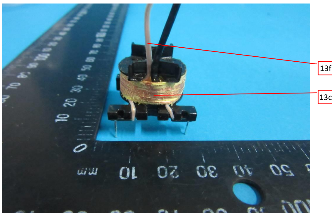
Photo 48 - Transformer for GT*96600-*56*** series
