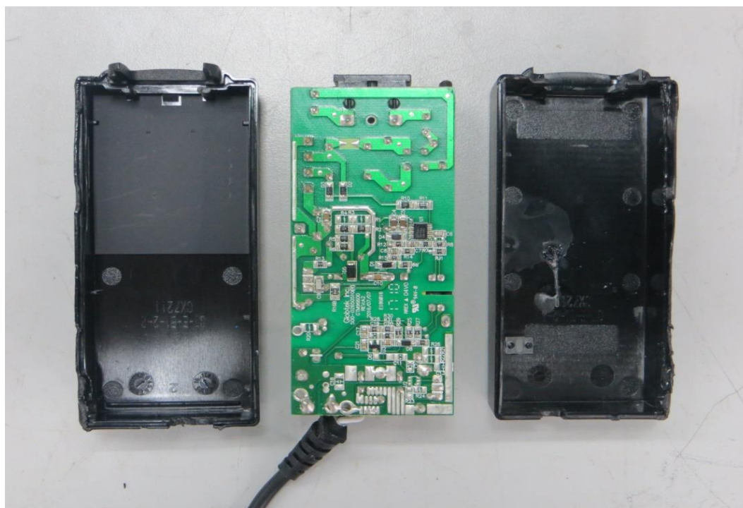
Photo 10 - Internal view
