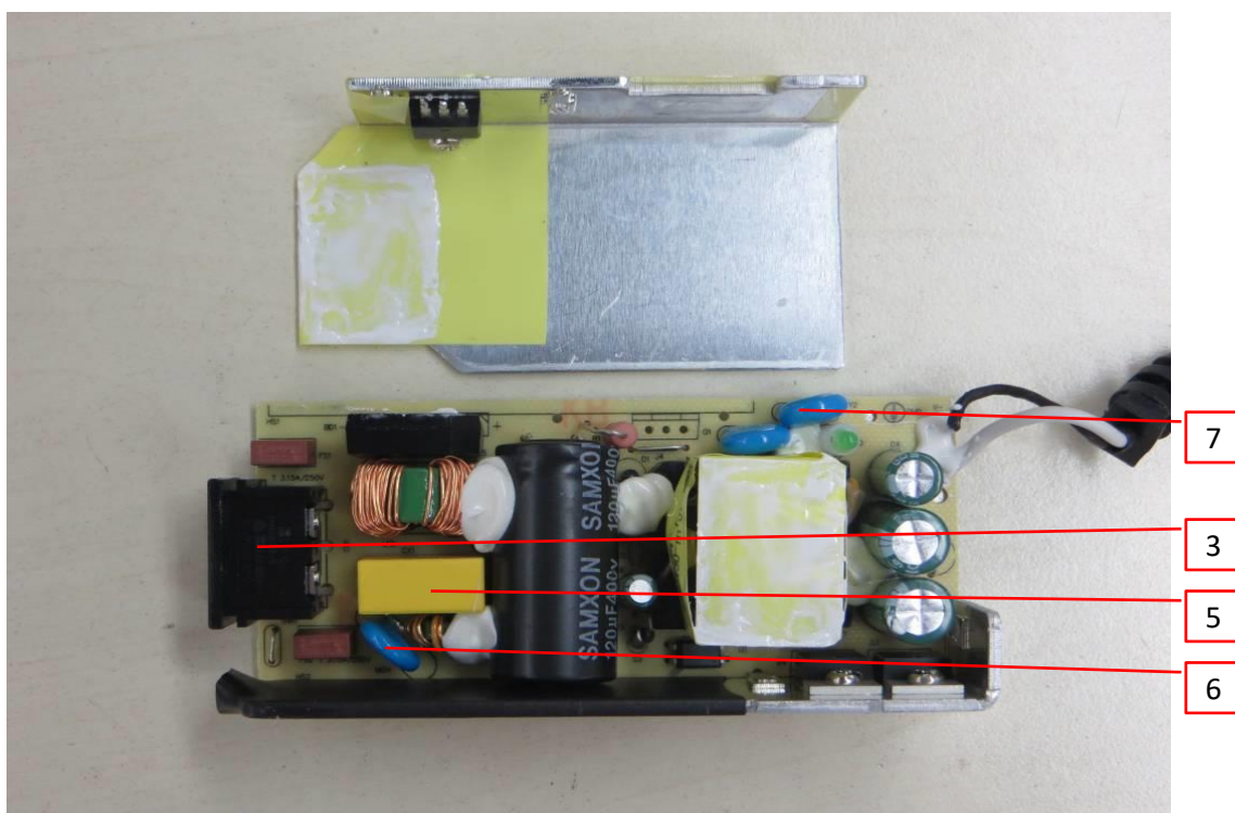
Photo 11 - PCB view
