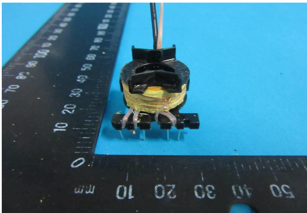
Photo 49 - Transformer for GT*96600-*56*** series
