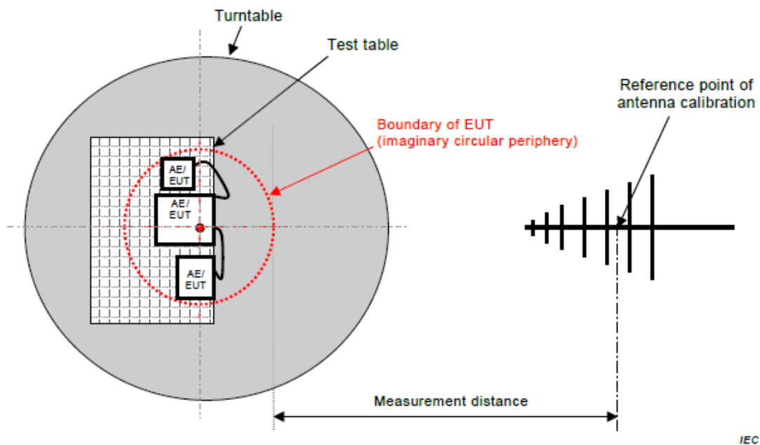
Figure C.1 – Measurement distance
