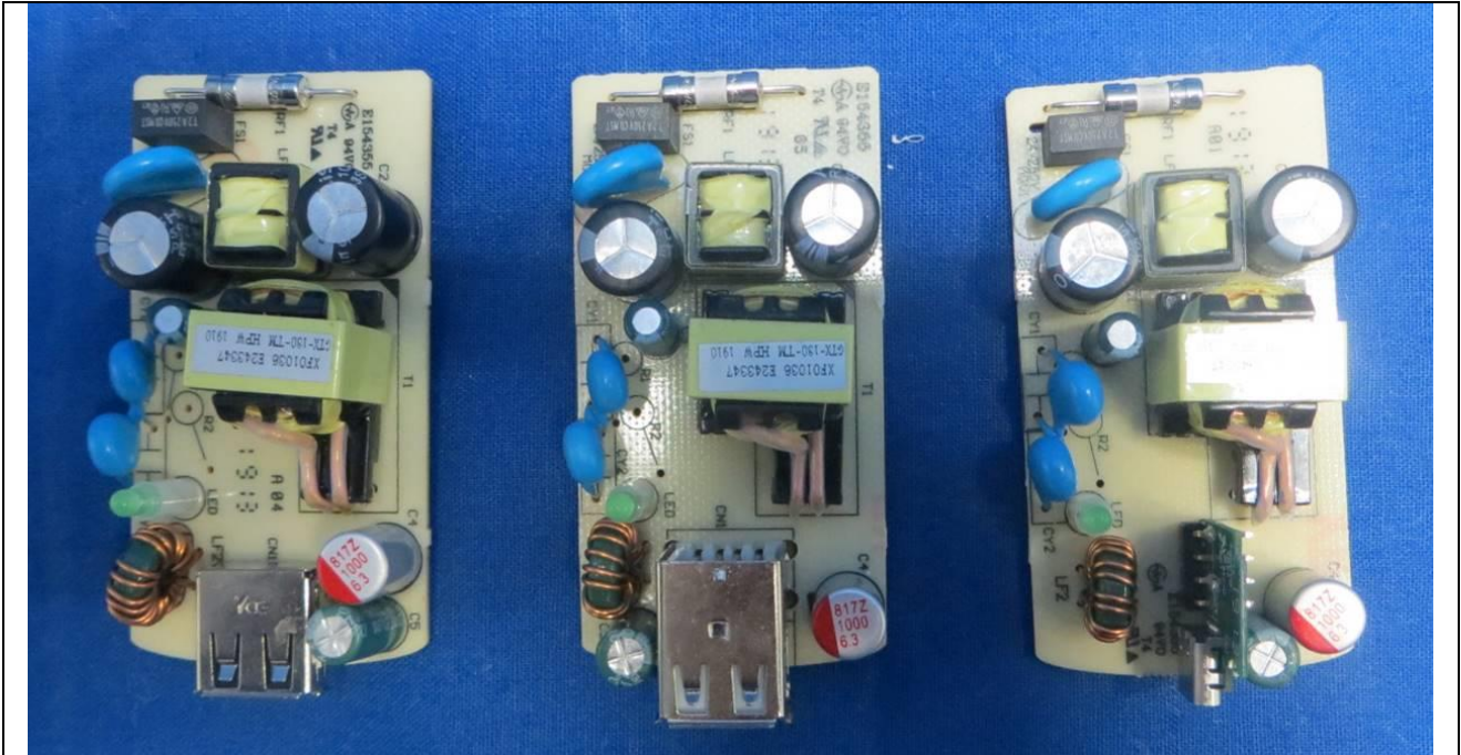
PCB (Type 2)
