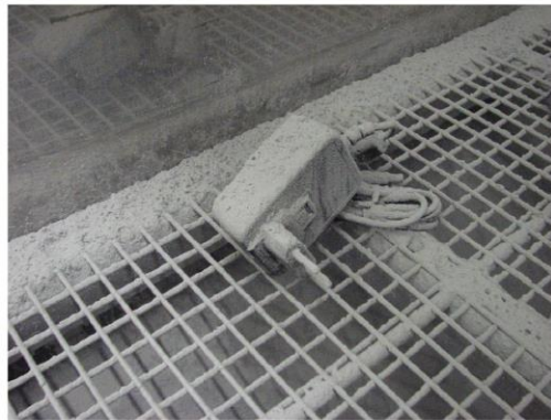
Figure 7: EUT after the dust test
