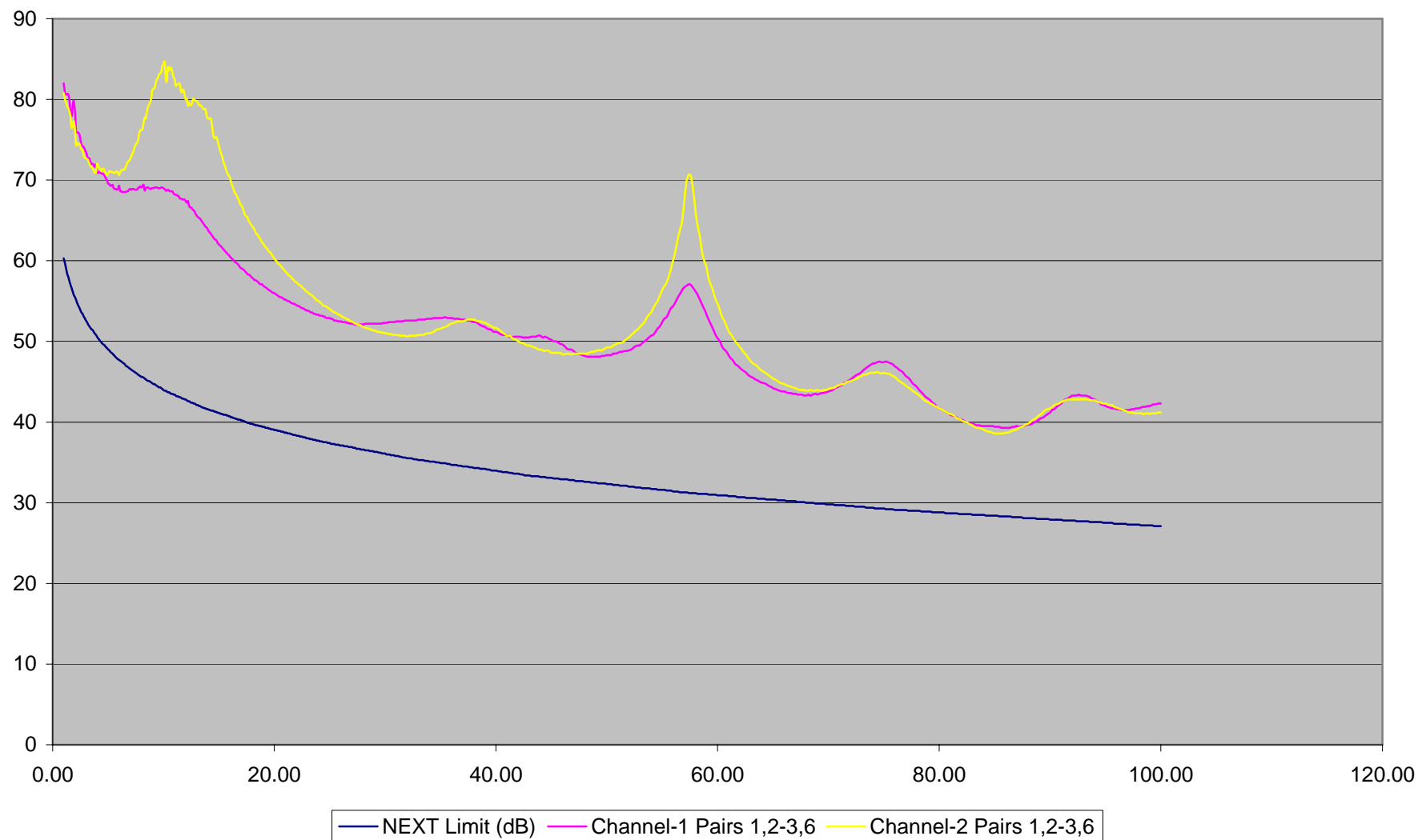
CAT 5 - TSB95 Spec @ Low Attenuation - Near End Cross Talk X-Axis Frequency (MHz), Y-Axis NEXT (dB)
