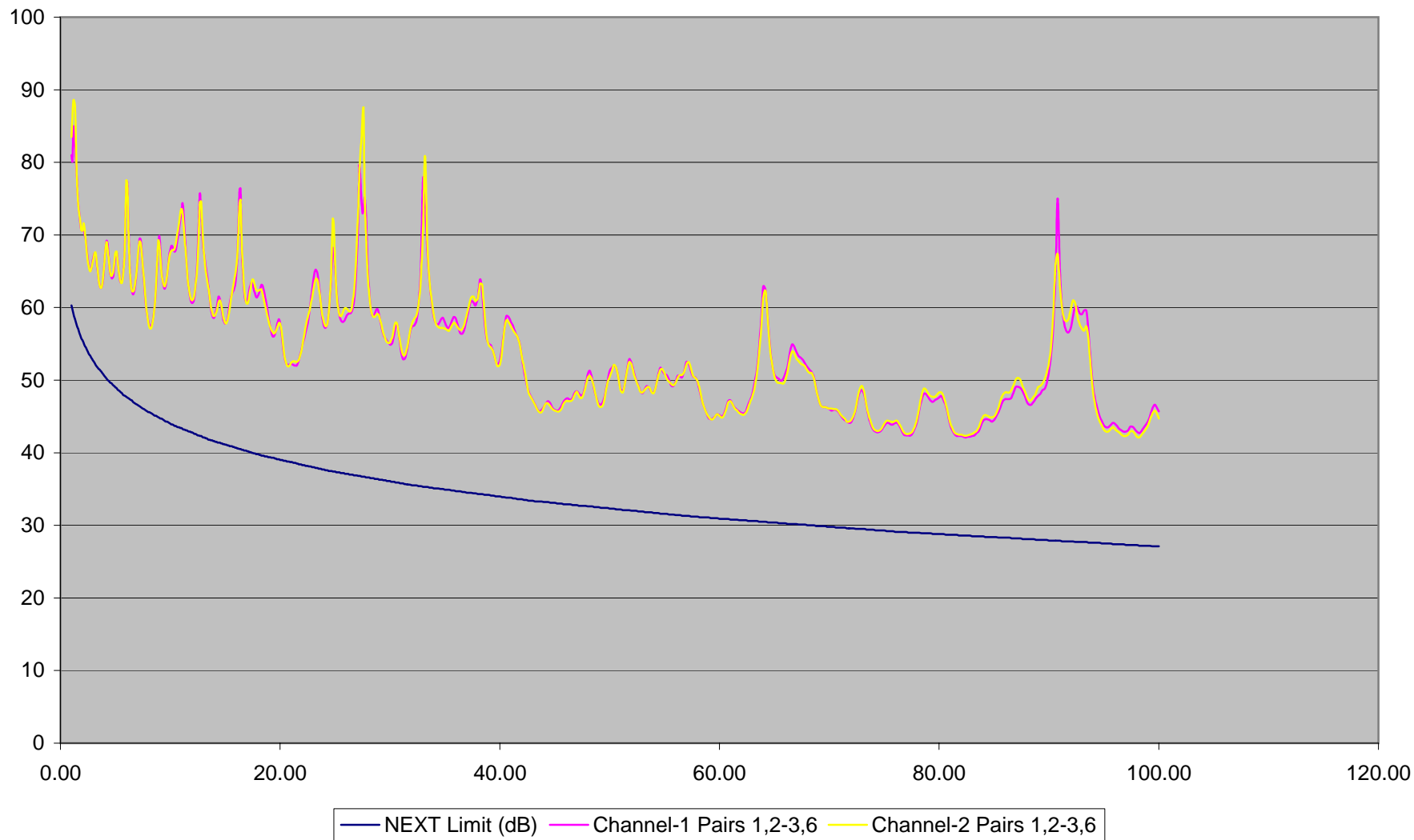
CAT 5 - TSB95 Spec @ Maximum Attenuation - Near End Cross Talk X-Axis Frequency (MHz), Y-Axis NEXT (dB)
