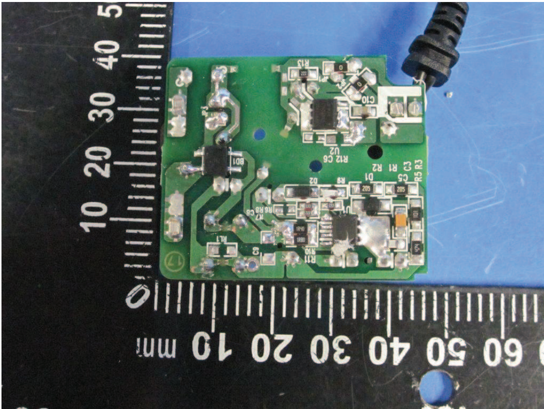
Picture 13 PCB B (configuration for LF1, LF2, CY1, see report description)
