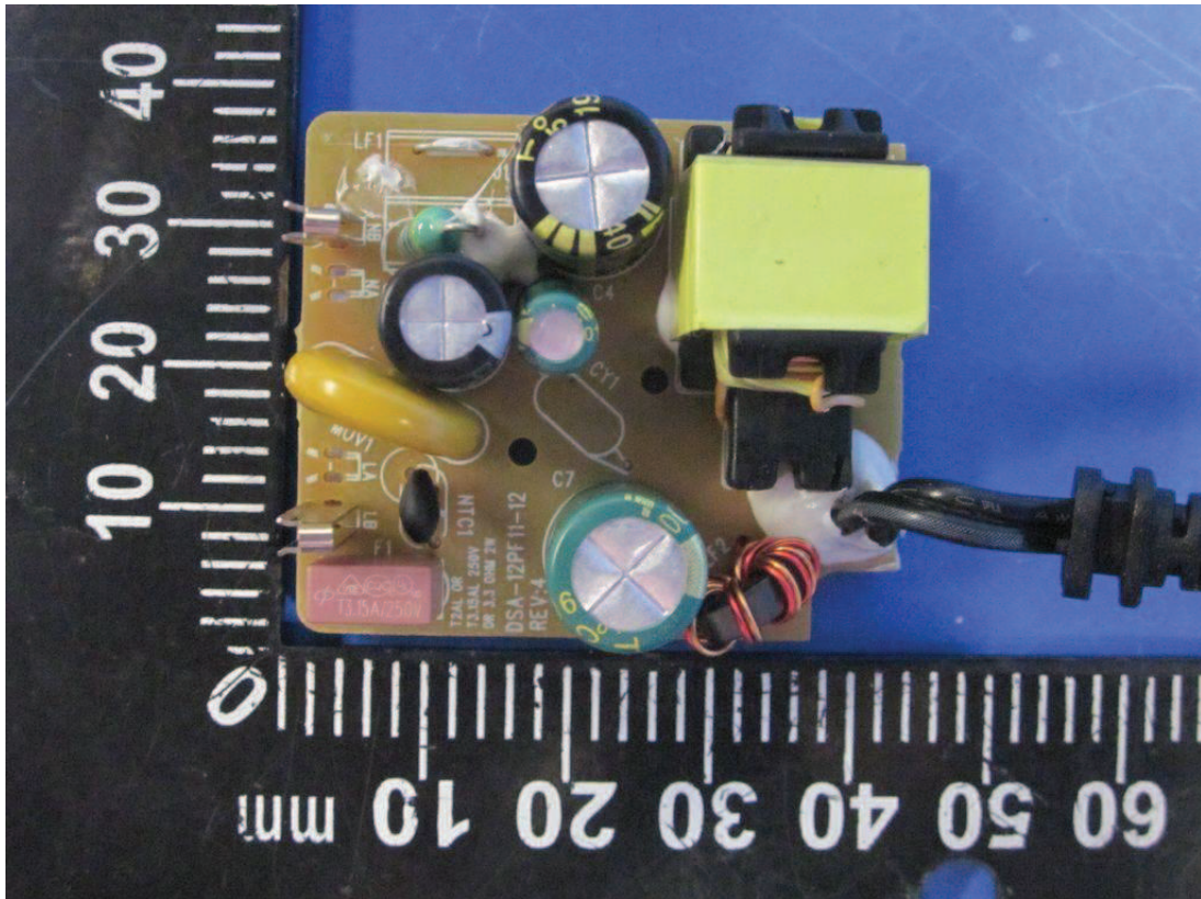
Picture 7 PCB A, Difference mode LF1, LF2, without CY1
