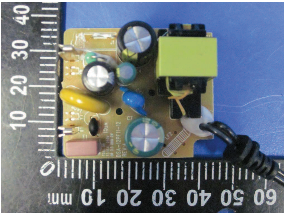
Picture 10 PCB A, Difference mode LF1, without LF2, with CY1
