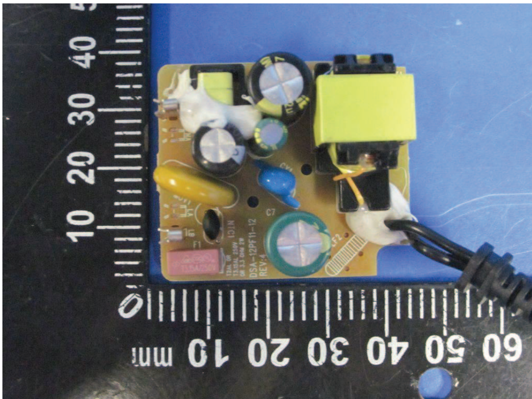
Picture 8 PCB A, Common mode LF1, without LF2, with CY1
