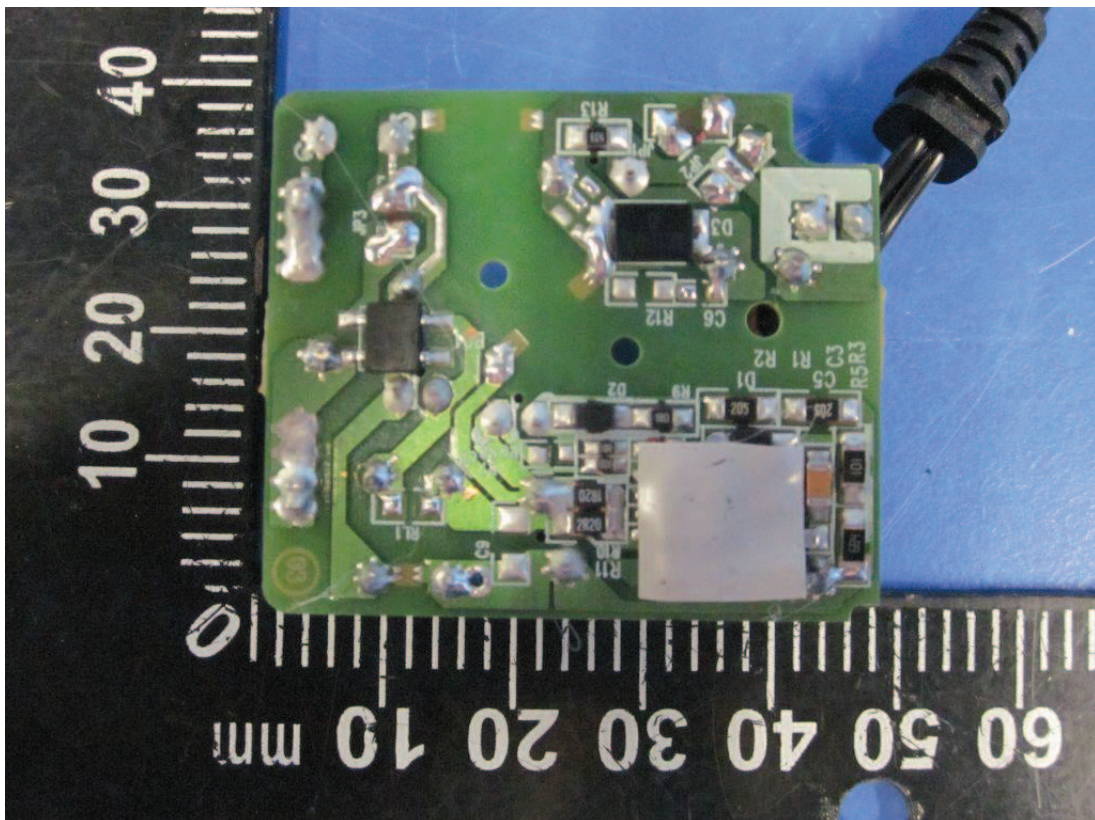
Picture 6 PCBA
