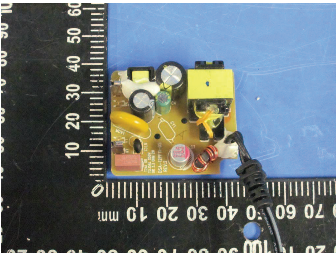
Picture 12 PCB B (configuration for LF1, LF2, CY1, see report description)
