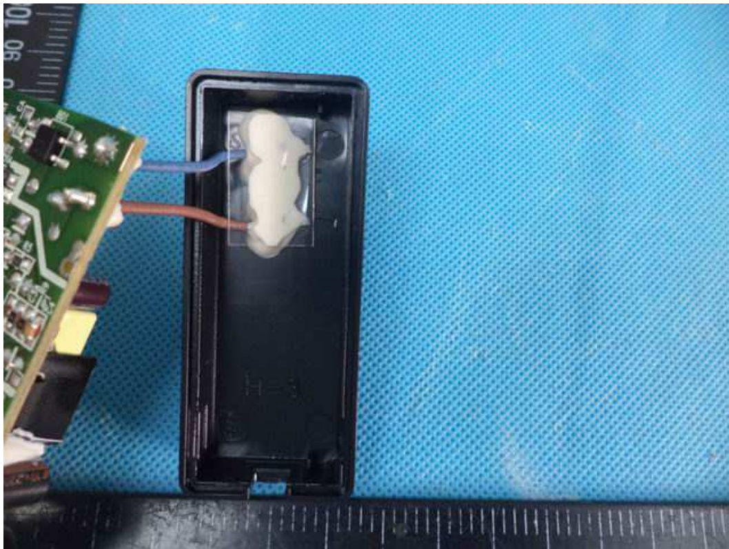
Photo 17 – Internal view of model GT-86120-WWVV*W2Z (US, JP, TAIWAN plug)
