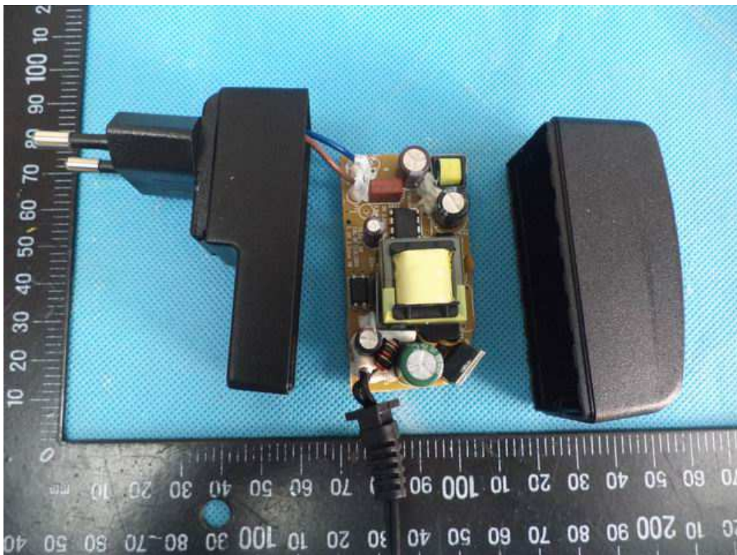
Photo 30 -- Internal view of model GT-86120-WWVV
