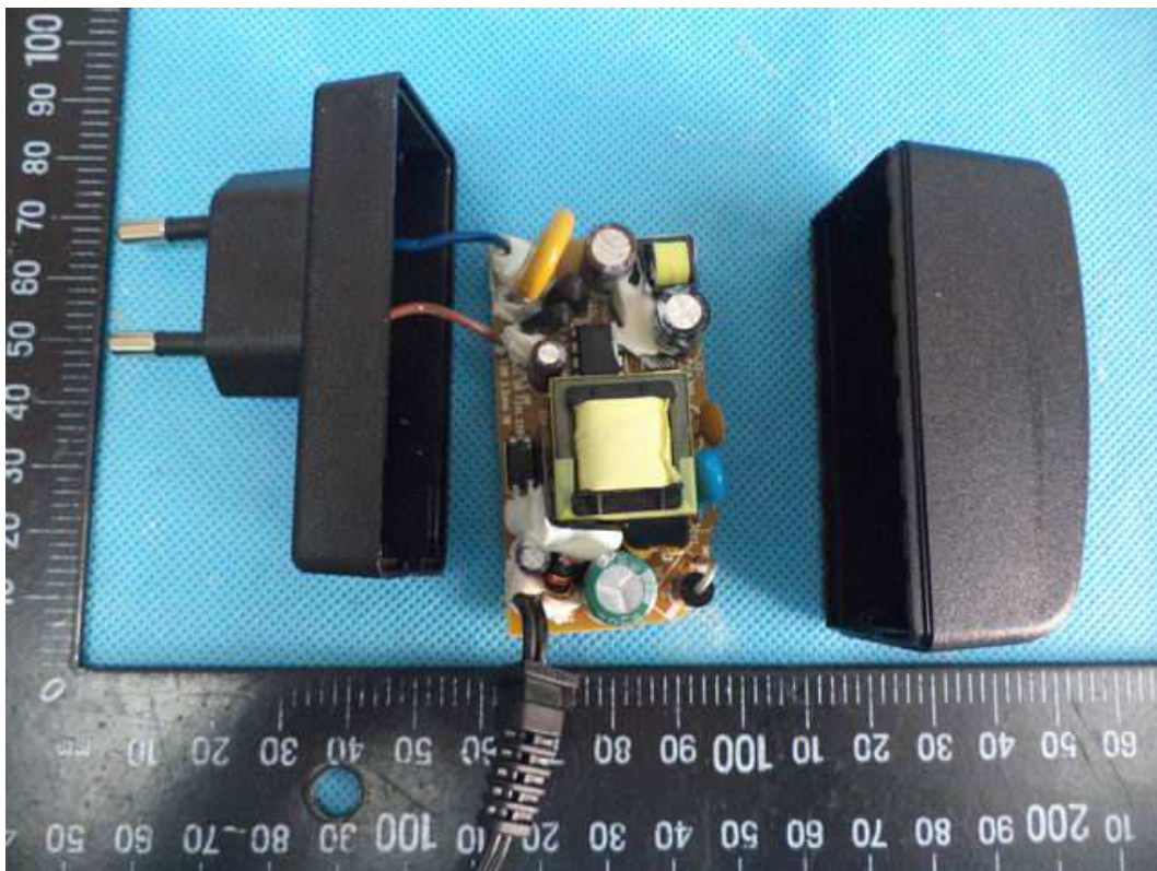
Photo 4 – Internal view of model GT-86120-WWVV*W2Z (with PCB type A) (EU plug)
