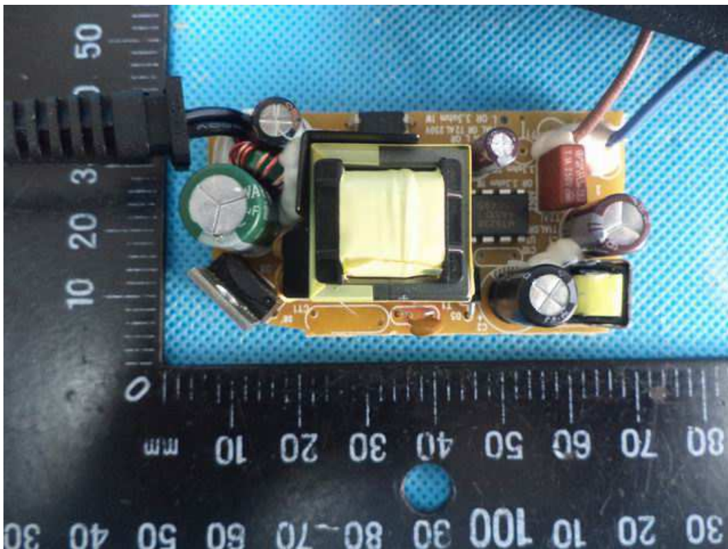
Photo 6 -- PCB view (PCB type A)
