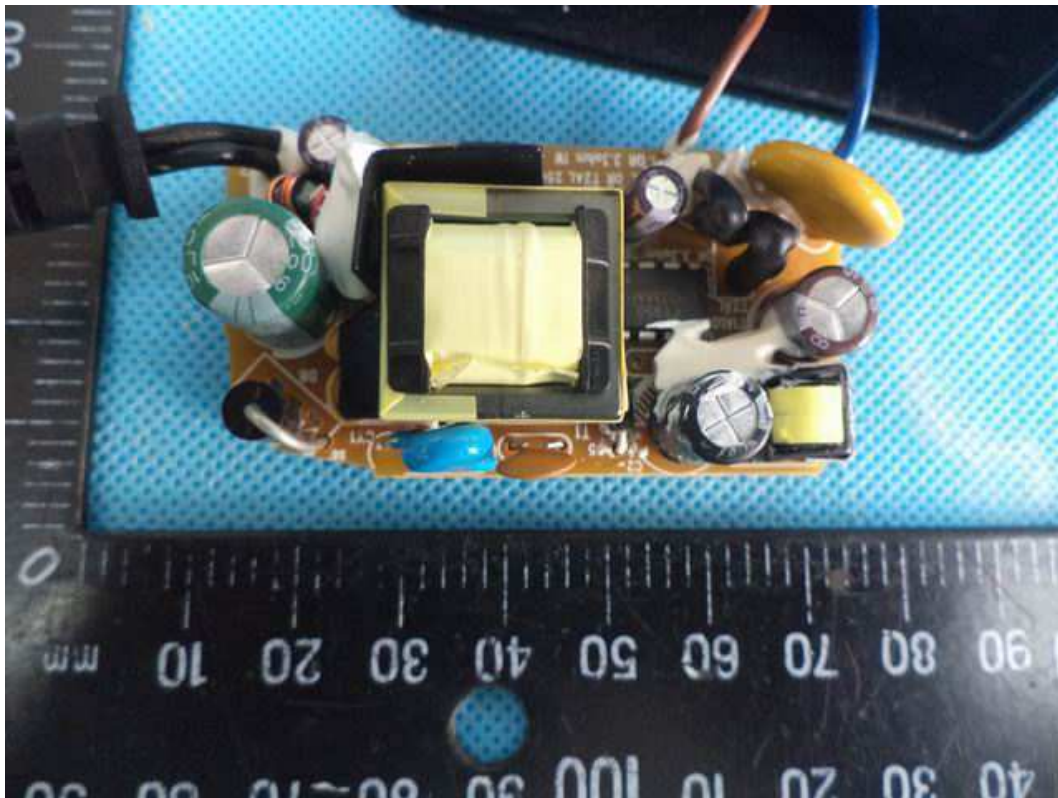
Photo 5 -- PCB view (PCB type A)
