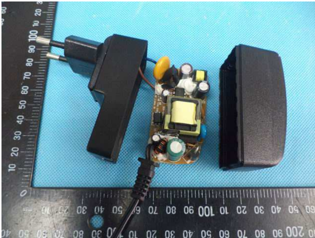
Photo 29 -- Internal view of model GT-86120-WWVV
