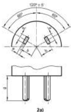
Figure 2 - Measures of the plug
