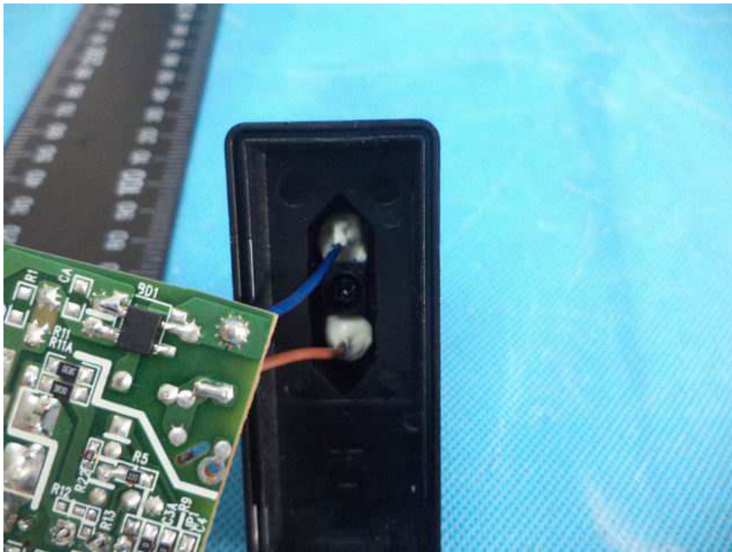
Photo 3 – Internal view of model GT-86120-WWVV*W2Z (with PCB type A) (EU plug)
