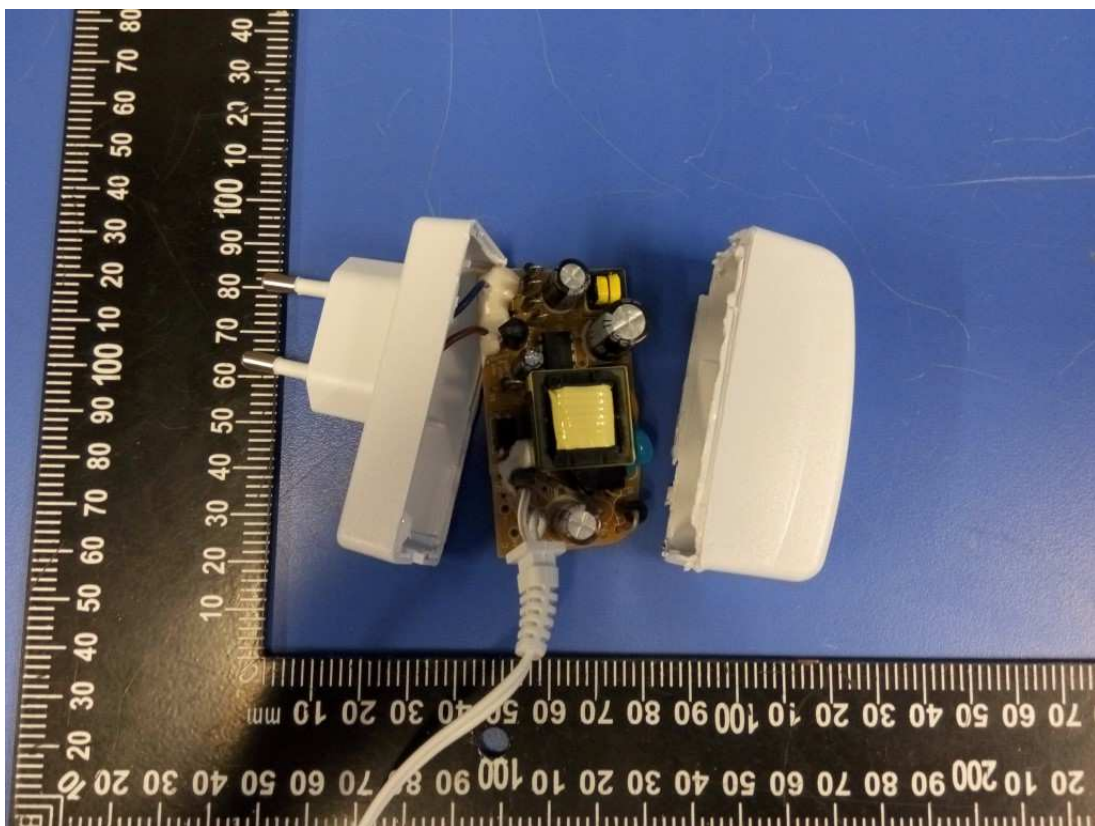
Photo 40 – Internal view of model GT-86120-1212*W2Z (With alternative PCB type B)
