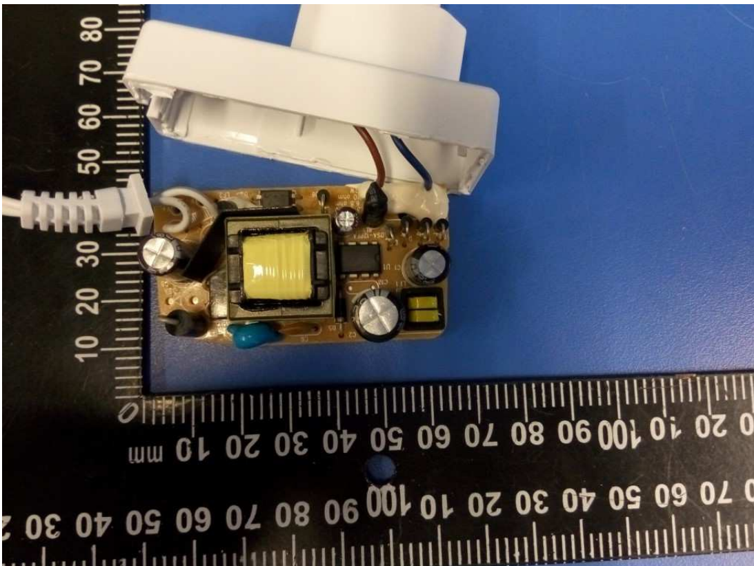
Photo 42 – Internal view of model GT-86120-1212*W2Z (With alternative PCB type B)
