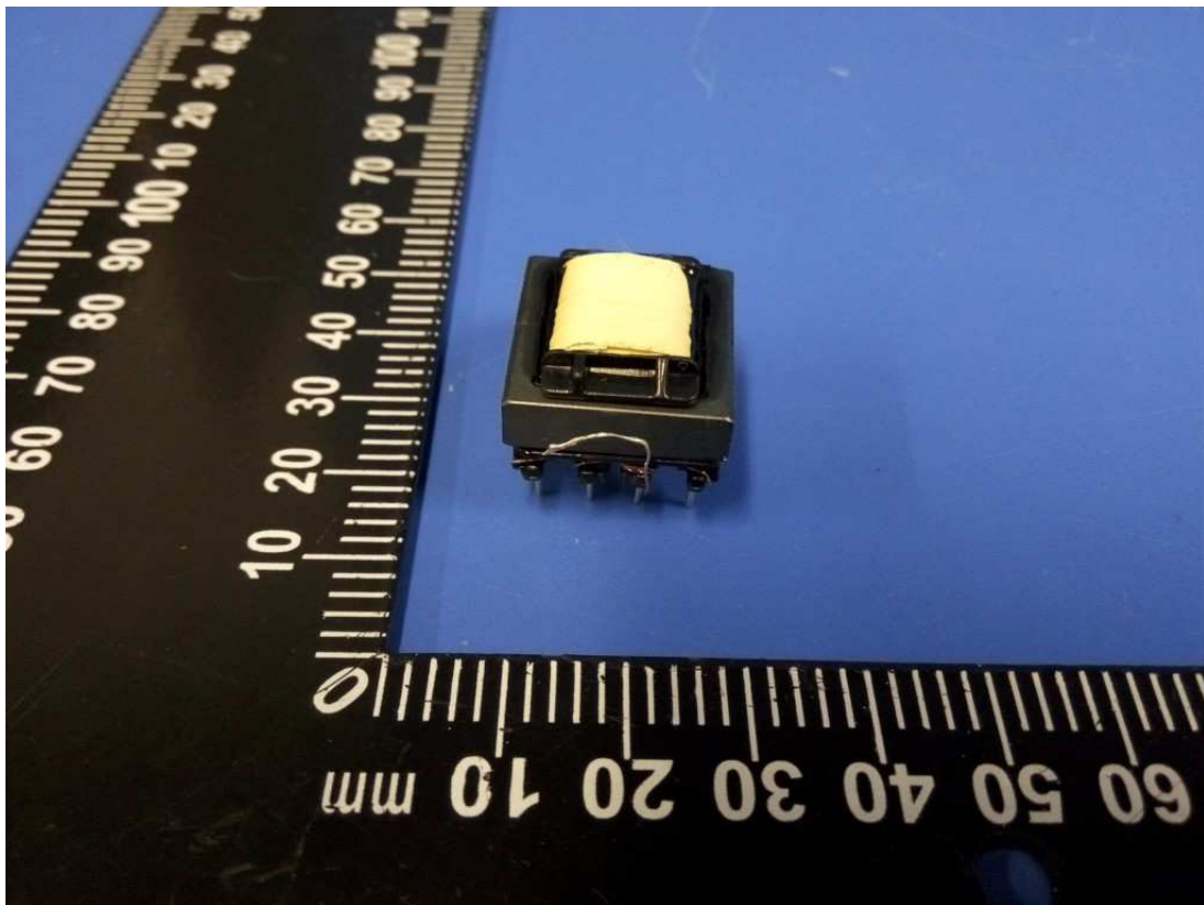
Photo 48 – Transformer view of model GT-86120-1212*W2Z (With alternative PCB type B)
