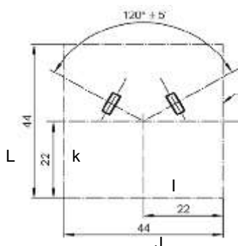
Figure 2 - Measures of the plug
