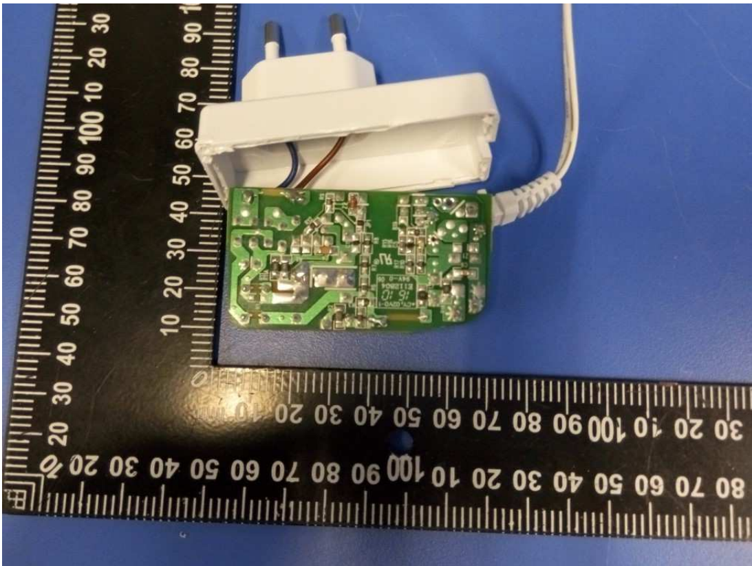
Photo 43 – Internal view of model GT-86120-1212*W2Z (alternative PCB type B)
