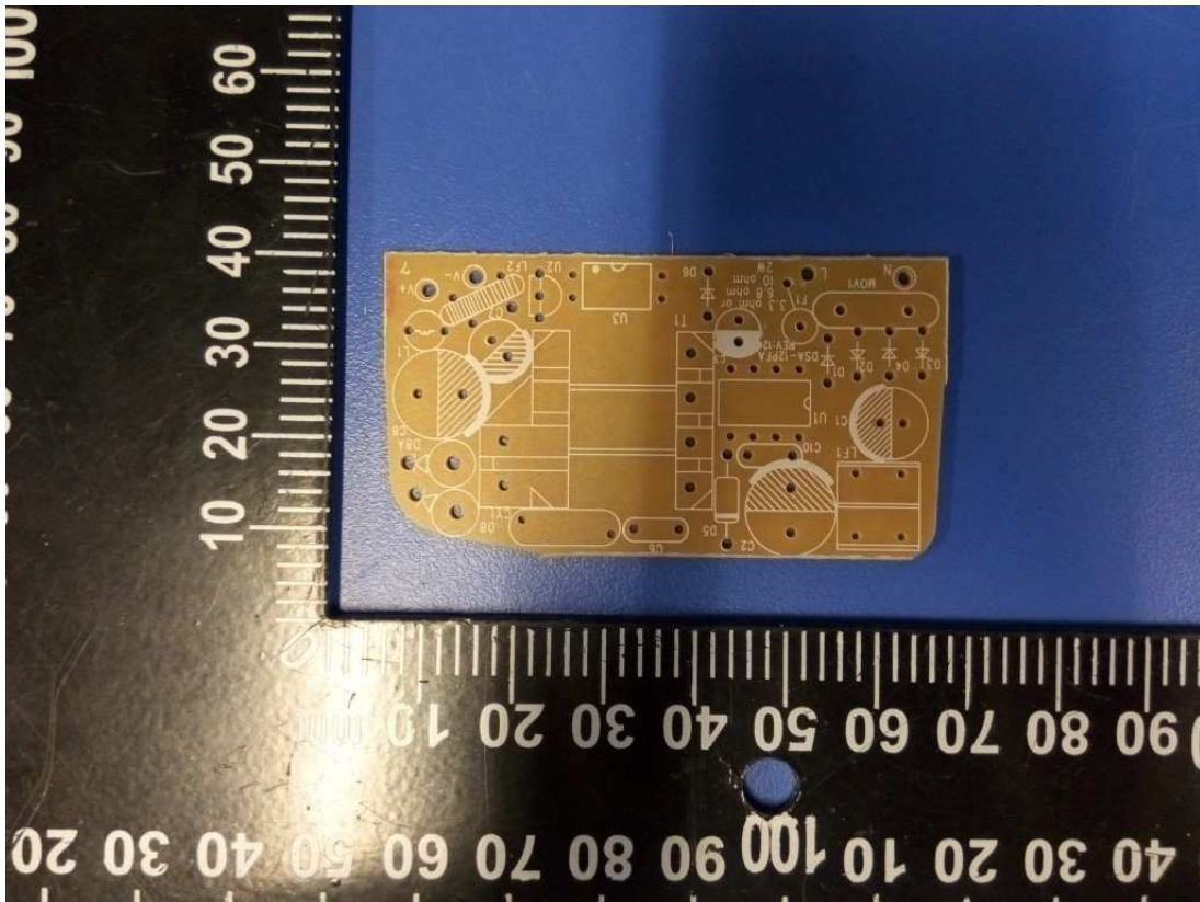
Photo 45 – PCB view of model GT-86120-1212*W2Z (alternative PCB type B)
