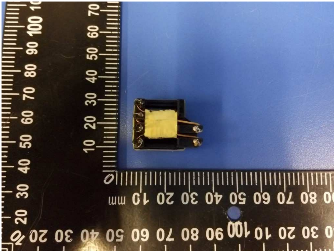
Photo 47 – Transformer view of model GT-86120-1212*W2Z (With alternative PCB type B)
