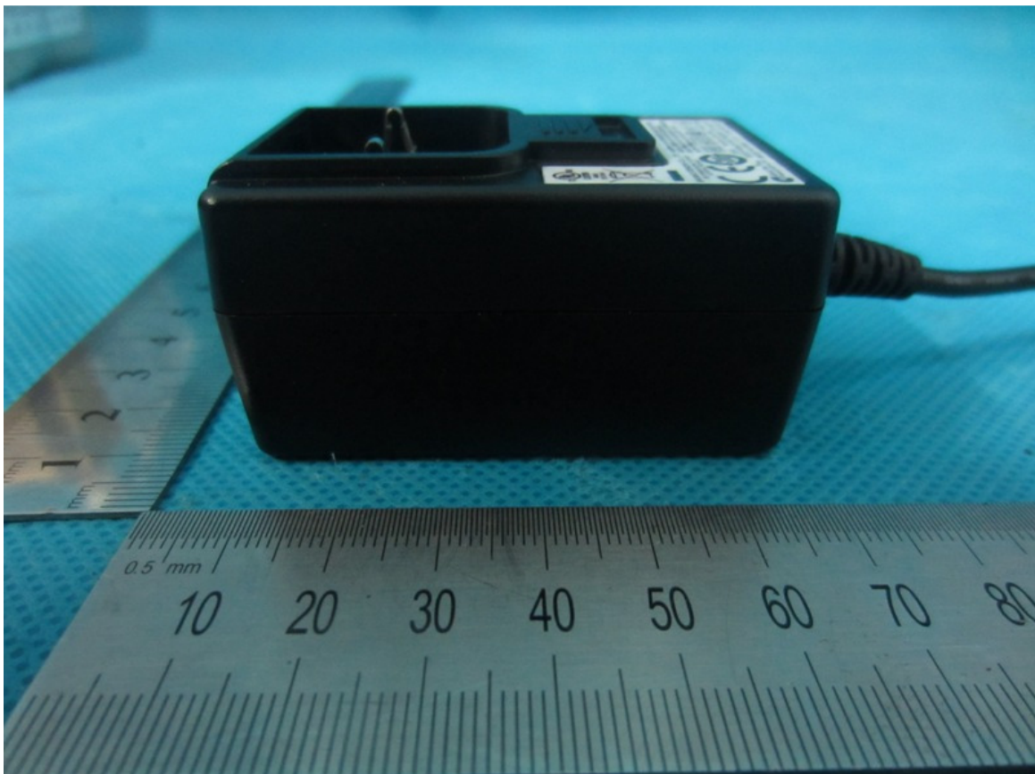
Side view
