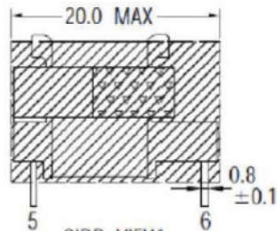
SIDB VIEW
