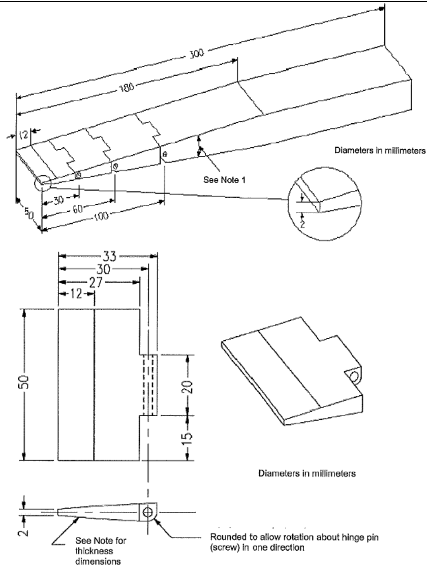
Details of the tip of wedge
