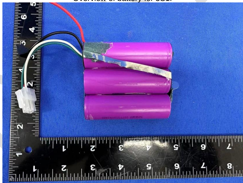
Photo 16 Overview of battery for 3S1P
