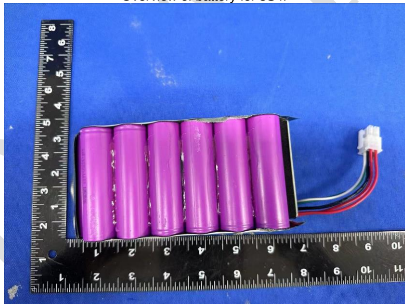
Photo 20 Overview of battery for 3S4P
