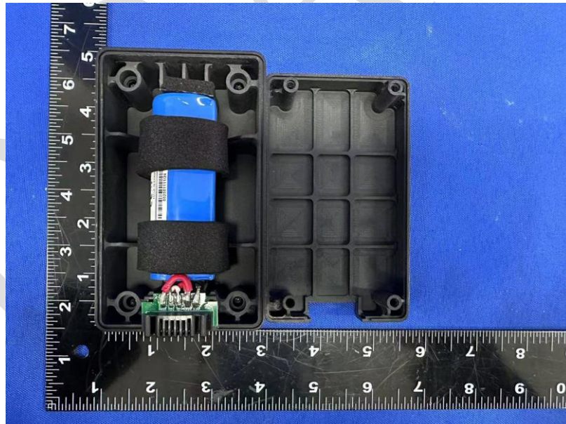
Photo 32 Overview of battery for 1S1P- Battery with case
