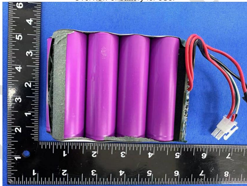
Photo 18 Overview of battery for 3S3P
