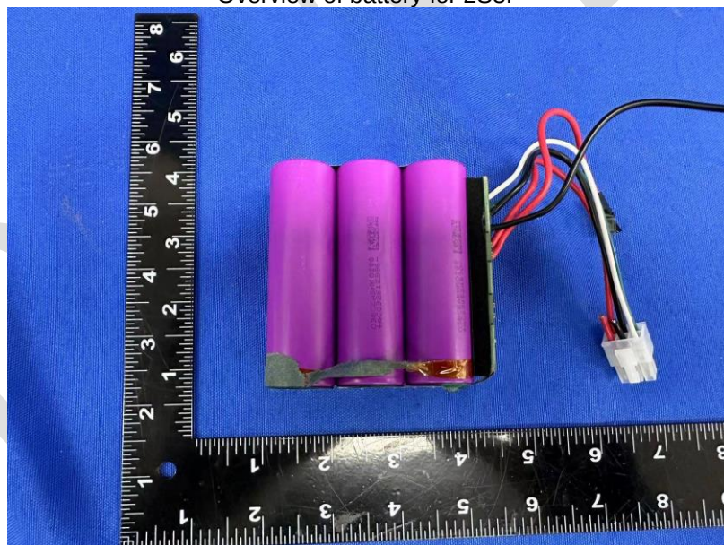
Photo 12 Overview of battery for 2S3P
