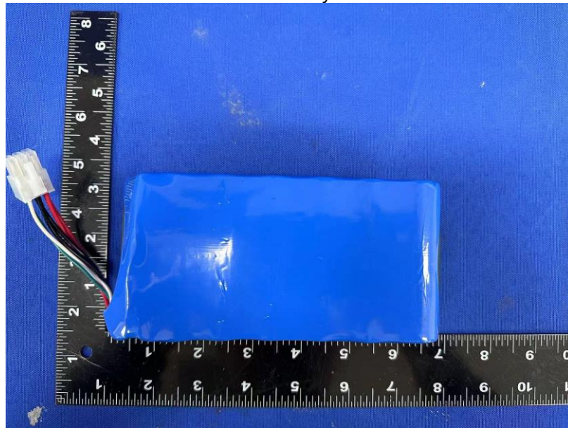
Photo 19 Overview of battery for 3S4P
