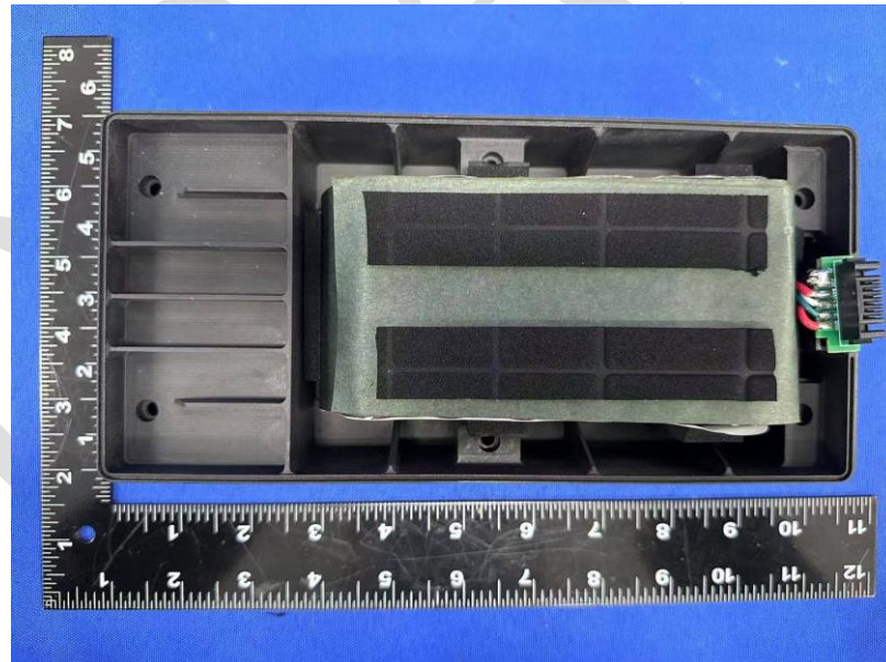
Photo 60 Overview of battery for 4S4P- Battery with case
