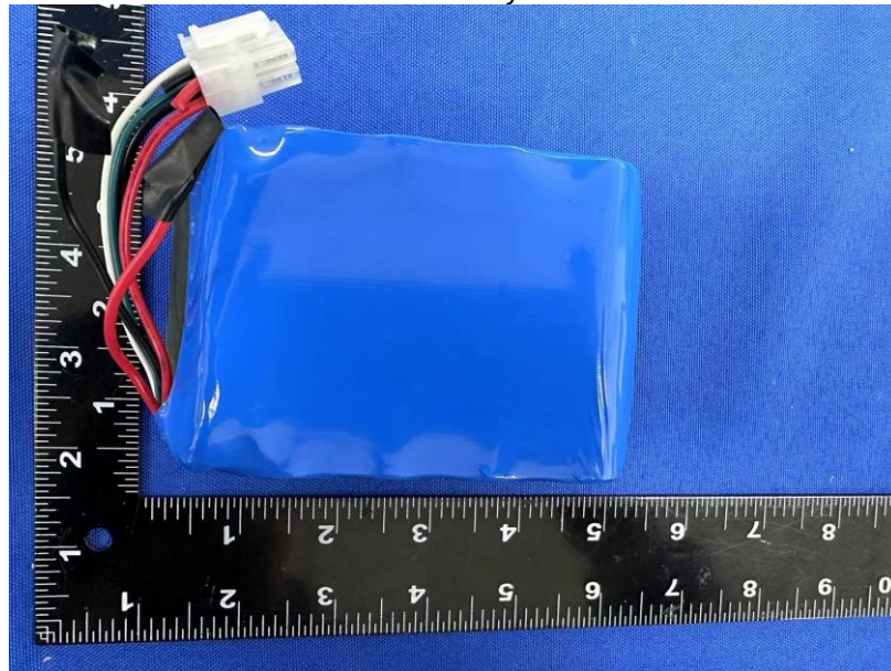
Photo 17 Overview of battery for 3S3P
