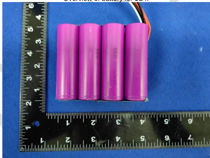
Photo 6 Overview of battery for 1S4P
