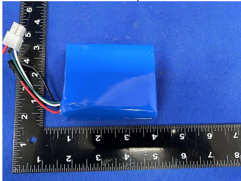
Photo 15 Overview of battery for 3S1P
