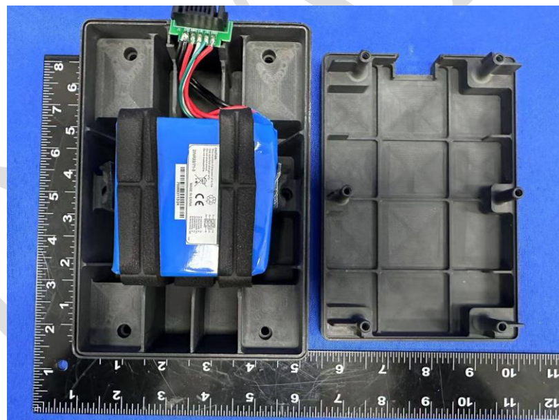
Photo 44 Overview of battery for 2S3P- Battery with case
