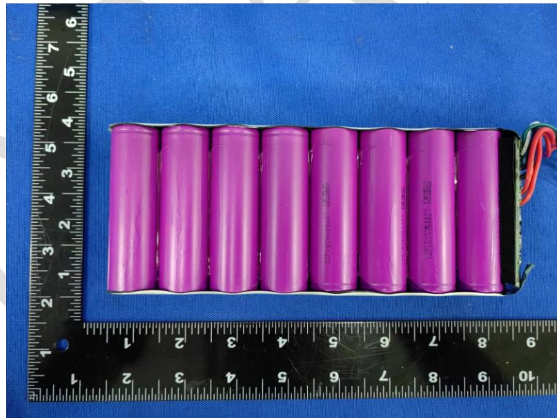
Photo 62 Overview of battery for 4S4P- Battery with case
