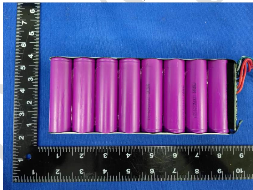
Photo 26 Overview of battery for 4S4P
