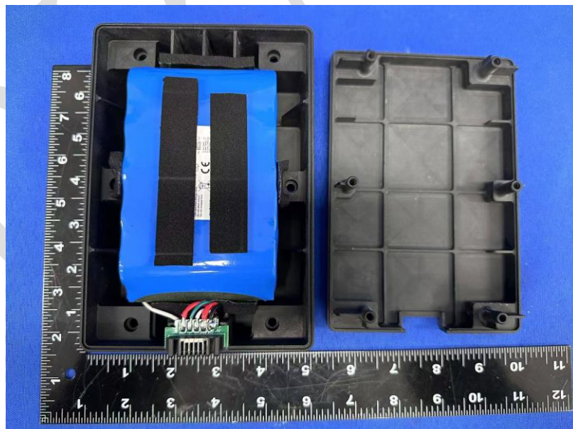
Photo 48 Overview of battery for 3S3P- Battery with case
