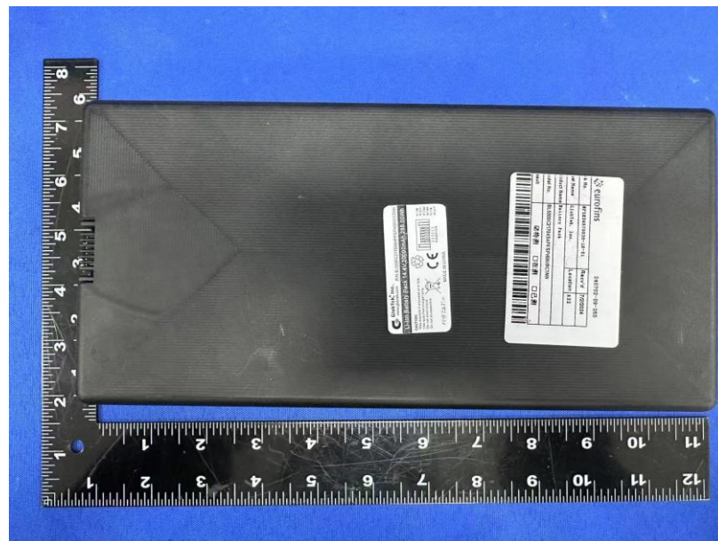
Photo 59 Overview of battery for 4S4P- Battery with case
