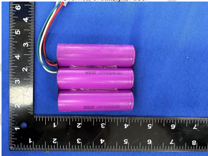
Photo 4 Overview of battery for 1S3P
