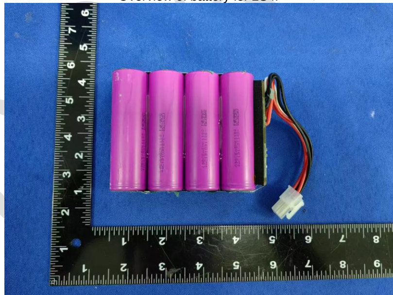
Photo 14 Overview of battery for 2S4P
