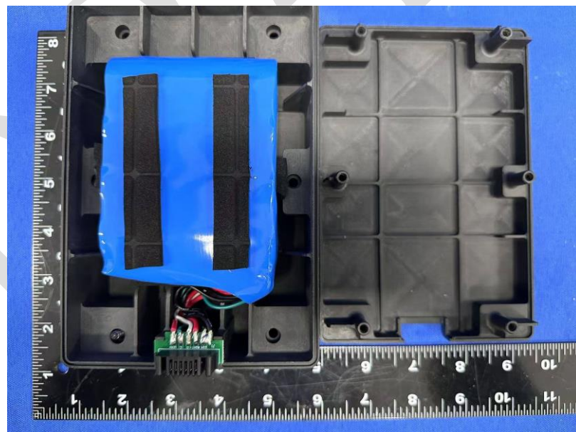
Photo 52 Overview of battery for 4S2P- Battery with case
